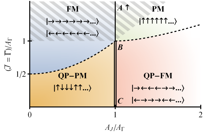
FIG. 1: Phase diagram. The hatched region defines the weakly modulated regime with no weak coupling ( J(Qi), \Gamma(Qi) > 0 \forall i ). The usual gapped ferromagnetic (blue) and paramagnetic (green) phases appear in this regime, separated by a continuous transition in the clean Ising class (segment AB ). At stronger modulation, we find two new modulated gapless phases: the QP-PM (yellow), and the QP-FM (red). The continuous transitions out of these phases (double and dashed lines) are in the new QP Ising class.
