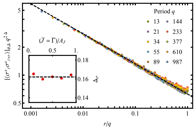
FIG. 4: Finite size scaling of spin correlations : (main) The average spin correlations q^{2\Delta_{\sigma}} [\langle \sigma_i^x \sigma_{i+r}^x \rangle]_{i,\phi,\Delta} collapse when plotted versus fractional separation r/q for critical dimension \Delta_{\sigma} \approx 0.16 at (J = \Gamma)/A_J = 0.5 . (inset) Least median deviation fit exponent \Delta_{\sigma} is stable along the segment BC consistent with universality.
