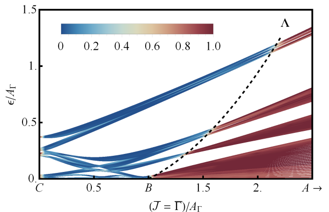
FIG. 2: Localisation properties of excitation spectrum on line ABC . The low-energy excitations on the segment AB are extended (red) up to a finite energy cut-off \Lambda , above which they are localised (blue). The cutoff \Lambda vanishes at the multicritical point B so that all finite energy excitations are localised on the segment BC . The color quantifies the scaling of the inverse participation ratio I = \sum_i |\psi_i|^4 \sim q^{-a} ; a = 0 (1) for localised (extended) states. Parameters: q = 233 , \Delta = 42\pi/233 , \phi = \sqrt{2}
