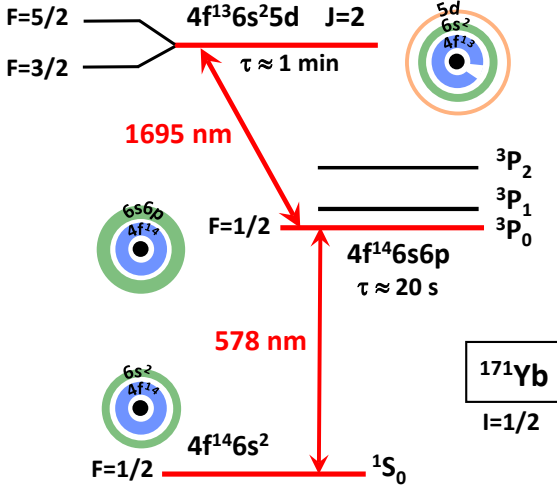
FIG. 1: Yb energy level scheme illustrating the 4f^{14}6s^2 \ ^1S_0 - 4f^{14}6s6p \ ^3P_0 and 4f^{14}6s6p \ ^3P_0 - 4f^{13}6s^2 5d (J=2) clock transitions. The open 4f shell of the J=2 state leads to the particularly high \alpha -sensitivity. Energies are not to scale.
