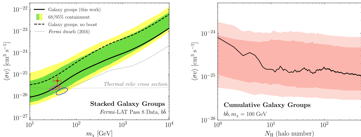
FIG. 1. (Left) The solid black line shows the 95% confidence limit on the DM annihilation cross section, \langle\sigma v\rangle , as a function of the DM mass, m_\chi , for the b\bar{b} final state, assuming the fiducial boost factor [20]. The containment regions are computed by performing the data analysis multiple times for random sky locations of the halos. For comparison, the dashed black line shows the limit assuming no boost factor. The Fermi dwarf limit is also shown, as well as the 2\sigma regions where DM may contribute to the Galactic Center Excess (see text for details). The thermal relic cross section for a generic weakly interacting massive particle [45] is indicated by the thin dotted line. (Right) The change in the limit for m_\chi = 100 GeV as a function of the number of halos that are included in the analysis, which are ranked in order of largest J -factor. The result is compared to the expectation from random sky locations; the 68 and 95% expectations from 200 random sky locations are indicated by the red bands.
