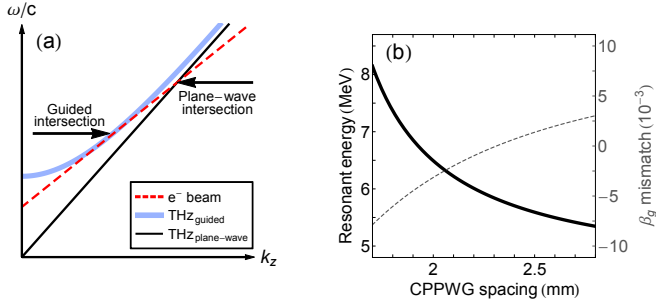
FIG. 2: (a) IFEL phase synchronism is given by the intersection between dispersion curves for electrons oscillating in the undulator (dashed red) and THz, for free-space plane-wave propagation (black) and waveguide propagation (light blue). Tangential intersection indicates group velocity matching (not to scale). (b) Resonant beam energy determined by CPPWG spacing using the parameters given in Table I at a single THz frequency (black). The corresponding group velocity mismatch is shown (dashed gray line with scale indicated on right axis).
