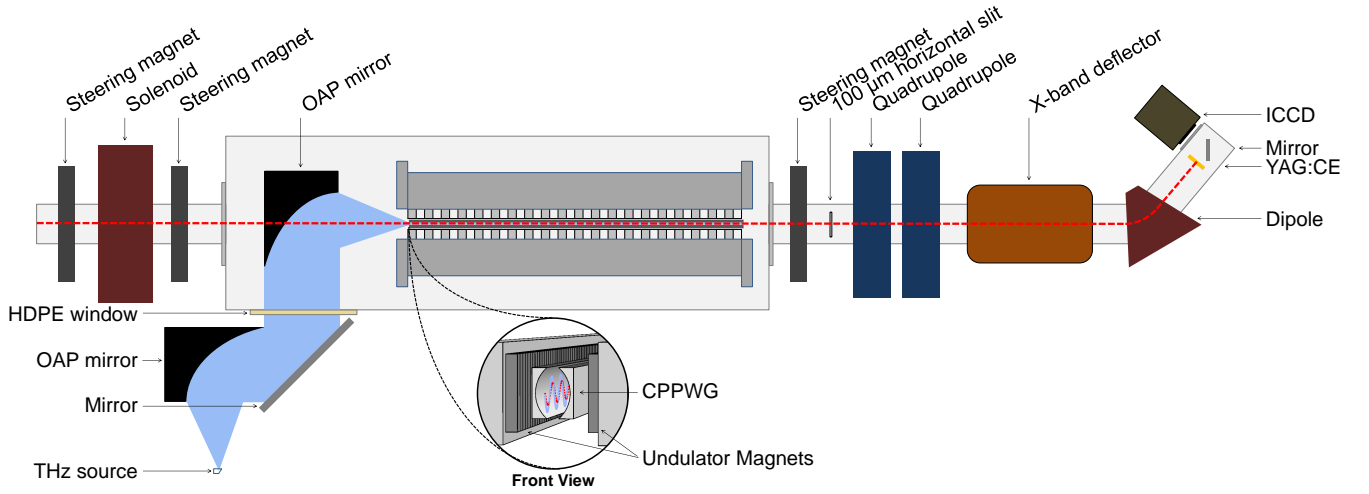
FIG. 1: Diagram of the experimental area on the PEGASUS beamline (not to scale), with inset view of the undulator entrance and curved parallel plate waveguide (CPPWG), showing electron beam (dashed red) and THz (light blue) path. THz radiation, generated via pulse-front-tilted optical rectification of 1 mJ of 800 nm laser in stoichiometric Lithium Niobate (sLN), was transported to the CPPWG using a system of off-axis parabolic (OAP) mirrors. A camera located outside the vacuum chamber imaged the CPPWG aperture, controlled via tunable 6-axis self-centering mount, to determine the spacing with 100 \mu\text{m} accuracy. A solenoid focused the beam through a 2 mm hole in the THz-focusing OAP to a 200 \mu\text{m} waist at the entrance of the planar Halbach style undulator. Downstream, a dipole magnet horizontally disperses the energy distribution onto a fluorescent high yield spectrometer screen. A 9.6 GHz transverse deflecting cavity could be used to streak the longitudinal beam profile onto the vertical axis.
