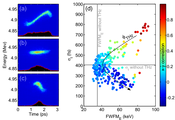
FIG. 5: LPS images showing the short beam (a) with positive energy chirp resulting in decompression, (b) unmodulated with THz off and (c) with negative energy chirp resulting in compression. The temporal distribution is projected at the bottom of each beam image. (d) Plot of rms bunchlength vs. energy spread, with color determined by energy-position correlation, for many LPS images. As expected, positive (warm) and negative (cool) correlation corresponds to decompression and compression of the beam, respectively. Gray lines show the mean energy spread and bunch length of the beam without THz interaction. An arrow highlights the transition in THz interaction phase from decompression to compression.
