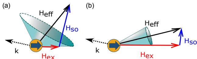
Figure 4. (Color online) Interplay between magnetism and intrinsic spin-orbit interaction. The spin of electron in Pt precesses around the effective field \vec{H}_{eff} = \vec{H}_{SO} + \vec{H}_{ex} , where \vec{H}_{SO} is the effective spin-orbit field determined by the electron's momentum \vec{k} , and \vec{H}_{ex} is the effective exchange field due to either proximity-induced magnetism or magnetic fluctuation in Pt. The electron's spin is shown by a bold circled arrow. (a) If H_{SO} dominates, precessional dephasing suppresses the spin polarization and/or magnetization fluctuation. (b) If H_{ex} dominates, the precession angle for electron spins aligned with \vec{H}_{ex} is small, suppressing the DP-like spin relaxation.
