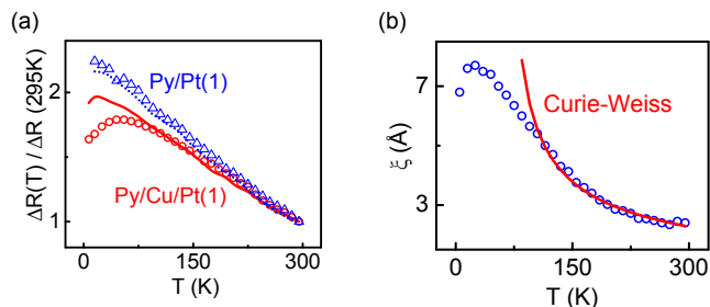
Figure 3. (Color online) (a) Measured (symbols) and calculated (curves) MR vs temperature for the standard spin valve nanopillar with d = 1 nm (circles and solid curve), and for the nanopillar with the structure Py(10)Pt(1)Cu(4)Py(5) (triangles and dotted curve). For the latter, the calculation includes only the EY contribution to spin relaxation. The MR is normalized by its value at RT. (b) Symbols: magnetic correlation length in Pt vs temperature, from Ref. [32]. Curve: dependence expected based on the Curie-Weiss law.
