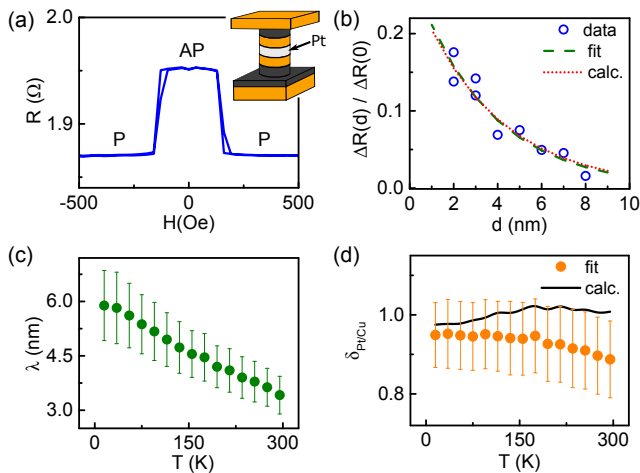
Figure 1. (Color online) (a) Resistance vs applied field for a sample without Pt spacer, at room temperature (RT), T = 295 K. Inset: schematic of the studied nanopillars, with Py layers shown in black, Cu in orange, and Pt in white. (b) Symbols: \Delta R , scaled by the MR of the reference sample without Pt spacer, vs Pt thickness d , at RT. Dashed curve: exponential fit to the data. Dotted curve: calculation based on the Valet-Fert theory. (c) Spin diffusion length vs temperature, determined by fitting \Delta R(d) with Eq. (1). (d) Interfacial spin-loss factor vs temperature, obtained by fitting \Delta R(d) with Eq. (1) (symbols), and by minimizing the difference between the MR data and the Valet-Fert calculations (curve).
