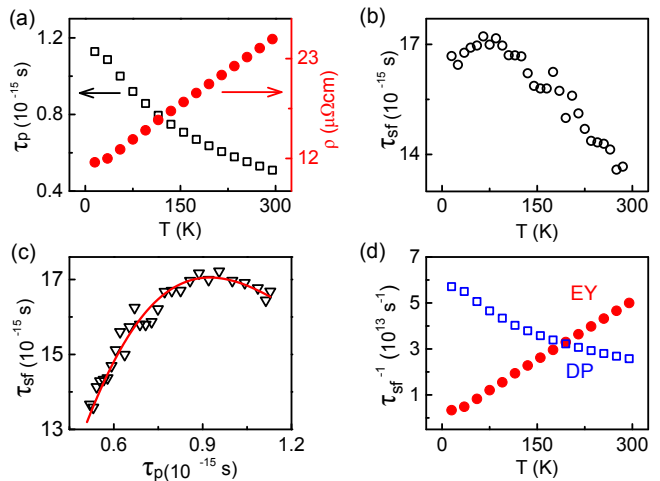
Figure 2. (Color online) (a) Bulk resistivity (right scale) and the momentum relaxation time (left scale) vs temperature for the studied Pt films. (b) Spin relaxation time vs temperature determined from the data of Fig. 1(c). (c) Spin relaxation time vs momentum relaxation time. Symbols: data, curve: fitting with a superposition of EY and DP-like contributions, as described in the text. (d) Temperature dependence of the contributions to spin relaxation from DP-like and EY mechanisms, as labeled, determined from the fitting in panel (c).
