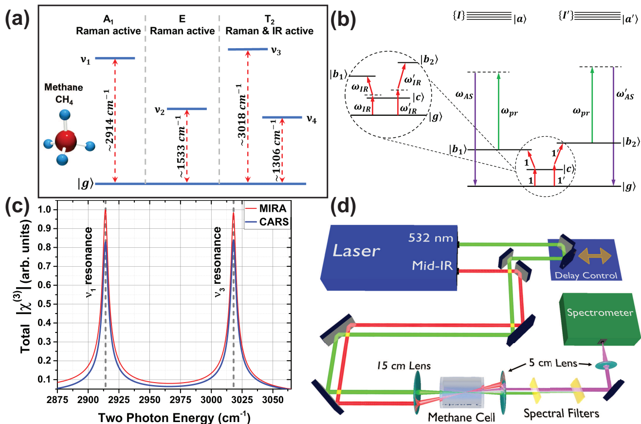
FIG. 2. (Color online) (a) Vibrational levels of methane. (b) MIRA CARS process for levels |b_1\rangle \equiv \nu_1 and |b_2\rangle \equiv \nu_3 via |c\rangle \equiv \nu_4 in methane. (c) Simulated magnitude of \chi^{(3)} as a function of detuning for an IR-enhanced Raman and traditional CARS schema. MIRA coherent Raman achieves a higher nonlinear susceptibility than traditional CARS. (d) Experimental Setup: The IR and 532 nm lasers travelled parallel throughout the beam path with \sim 1 cm separation, which translated to a 2\text{--}3^\circ angle between them when focused into the cell. The Stokes and anti-Stokes measurements used different spectrometers and spectral filters (see supplement).
