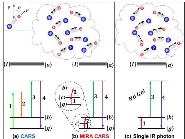
FIG. 1. (Color online) Two CARS schemes: (a) Typical CARS arrangement where \rho_{bg} coherence is generated by visible laser 1 and 2. (b) Mid IR Assisted (MIRA) CARS where \rho_{bg} is generated by mid-IR lasers 1 and 2. The photons at frequencies \omega_1 and \omega_2 do not need to be equal but could be chosen such that \omega_1 = \nu_{cg} and \omega_2 = \nu_{bc} . The two-photon excitation for both CARS and MIRA CARS produce a non-zero \rho_{bg} since all molecules vibrate “in phase”. The vibrations are shown schematically as stretching or compressing of the interatomic distance of the molecules. (c) Single photon excitation results in \rho_{bg} = 0 when averaged over all molecules since they vibrate “out of phase”. Inset The angle between the electric field ( E ) of the laser and the dipole \mu of molecule is defined as \theta .
