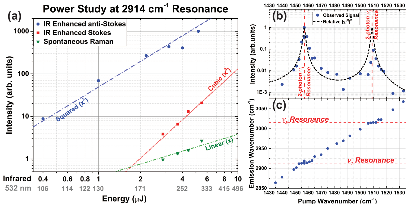
FIG. 3. (Color online) (a) Power dependence for the MIRA anti-Stokes and Stokes emission as well as the spontaneous Raman. The energies of both the 532-nm pump and IR field at 1457\text{ cm}^{-1} were varied simultaneously, as such both energies shown on the x-axis. (b) Intensity of observed emission as a function of spectral detuning via the IR laser. The change in Raman intensity qualitatively agrees with the expected values of |\chi^{(3)}|^2 . (c) Raman wavenumber versus IR pump wavenumber. The emission still occurs at the Raman transition wavenumber when the IR coupled field is slightly detuned from two-photon resonance.
