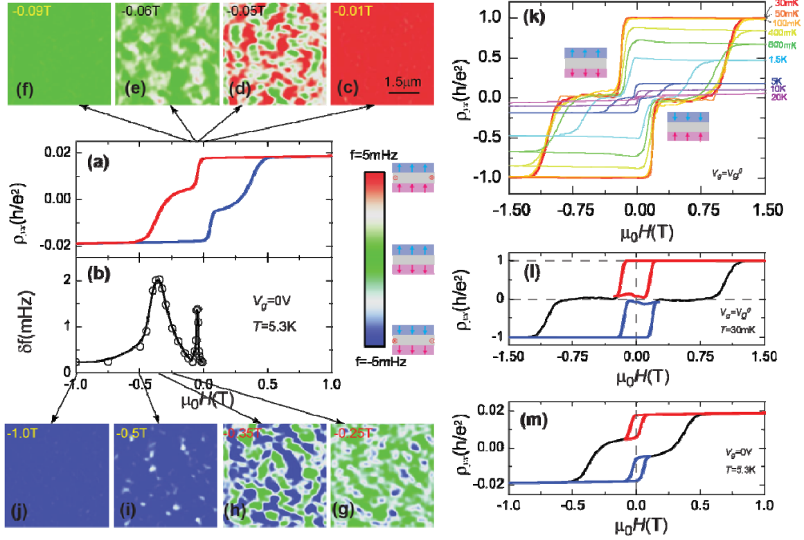
Figure 3| Two-step magnetization reversal in the 3-5-3 SH2. (a) \mu_0H dependence of \rho_{xx} of 3-5-3 SH2 at V_g=0V and T=5.3K . (b) \mu_0H dependence of magnetic domain contrasts ( \delta f ) at V_g=0 and T=5.3K . The \delta f is estimated from the root-mean-square (RMS) value of MFM images in (c-j). (c-j) The MFM images at various \mu_0H s. Red and blue represent respectively upward and downward parallel magnetization alignment regions, green represents antiparallel magnetization alignment regions. The Hall traces in (a) and the MFM images in (c-j) are measured simultaneously. (k) \mu_0H dependence of \rho_{yx} at various temperatures. \rho_{yx} exhibits two-step transition when T < 10K . (l, m) Minor loops of the \rho_{yx} at V_g=V_g^0 and T=30mK (l) and at V_g=0V and T=5.3K (m).
