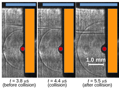
FIG. 4: Time evolution of the primary (spherical) and secondary (planar from top) solitons before, during, and after collision ( T = 1.7 K). The red circle indicates the origin for the primary wave emission and the top (blue) surface for the secondary wave. The delay between the ablation and back-light laser pulses is indicated by t .
