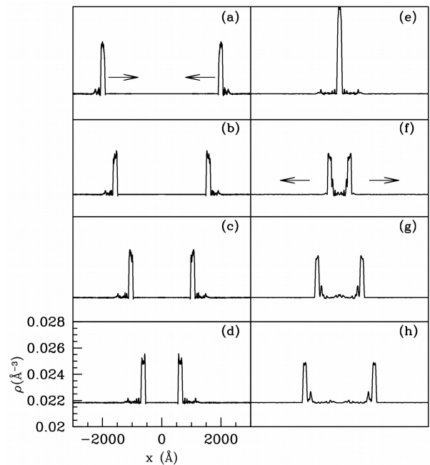
FIG. 5: Snapshots of superfluid ^4\text{He} density along the direction of soliton propagation ( x -axis) from TDDFT. The initial compression was created on the simulation box boundary with n = 30 (see text). Due to periodic boundary condition, the solitons propagate as shown in (a) - (d), collide in (e), and continue propagating almost unchanged in (f) - (h). When compared with experiments, the x -axis is oriented perpendicular to the ablation target.
