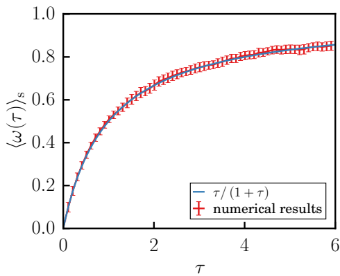
FIG. 2. Dependence of average steady-state entropy production rate \langle \omega(\tau) \rangle_s on the persistence time \tau for an active particle in a simple harmonic well. As in the case of Fig. 1, in the plot we have assumed mobility \mu and temperature T to be unity and a temperature scale that ensures k_B = 1 .
