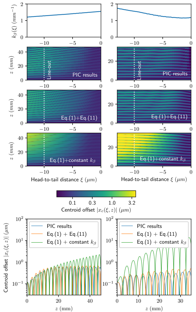
FIG. 2. Evolution of the centroid offset (log-scaled colormap) as a function of the head-to-tail coordinate \xi and the propagation distance z , for (case (a); left panels) a bunch driver with r_d = 4 \mu\text{m} , \ell_d = 3 \mu\text{m} , \xi_d = 27 \mu\text{m} and n_d = 0.7 n_p , and (case (b); right panels) a laser driver with a_0 = 0.4 , \tau = 20 \text{ fs} , \xi_d = 26 \mu\text{m} , w = 24 \mu\text{m} . The top plots show the head-to-tail variations of the betatron frequency k_\beta in both cases. The upper colormaps show results from the PIC simulations, while the middle and lower colormaps show results from the numerical integration of Eq. (1), with k_\beta(\xi) either given by Eq. (11) (middle colormaps) or considered uniform (lower colormaps). The lower plots are line-outs of the colormaps, at a fixed head-to-tail distance ( \xi = -10 \mu\text{m} ; indicated by a white dotted line on the colormaps).
