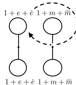
FIG. 4. Braid for the \wedge \sigma_3^z gate.
