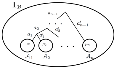
FIG. 1. Ground state for n gapped boundaries \mathcal{A}_i on a plane and total charge vacuum. All edges are directed to point downward.
