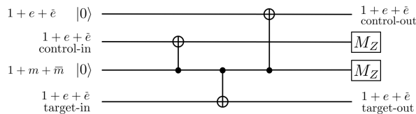
FIG. 5. Short circuit (generalizing Ref. [13]) to use three SUM gates between 1+m+\bar{m} and 1+e+\bar{e} qutrits to implement a SUM gate between 1+e+\bar{e} qutrits. All entangling gates drawn are \text{SUM}_3 .
