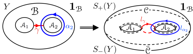
FIG. 3. Topological charge projection ( n = 2 ).
