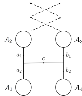
FIG. 2. Braiding of two gapped boundaries ( \sigma_2^2 ). Solid lines indicate tunneling operators from the basis vectors (i.e. not motion of the holes), while dotted lines indicate how the holes move in the braiding process.
