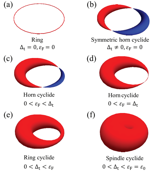
FIG. 1. Evolution of the Fermi surface (FS) as a function of tilt \Delta_t and Fermi energy \epsilon_F with red (blue) indicating the electron (hole) pocket. (a) At zero Fermi energy with zero tilt, the FS has a one dimensional ring shape sitting on the zero energy plane. (b) With a finite tilt, the ring shape evolves into symmetric horn cyclide containing both electron and hole pockets symmetrically, which vanish at two contact points. Upon increasing the Fermi energy, the electron and hole pockets (c) become asymmetric and the contact points move out from the symmetrical axis, (d) converging into a single point when the Fermi energy equals the tilt energy, and (e) vanish when the Fermi energy becomes larger than the tilt energy. (f) When the Fermi energy equals the energy scale of the ring radius, the FS is merged into a sphere-like shape with no holes in the center, similar to that of Weyl semimetals.
