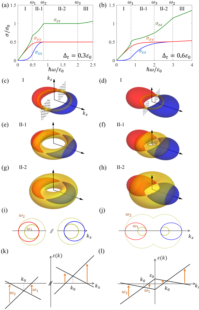
FIG. 3. (a), (b) Calculated optical conductivities of NLSMs for \varepsilon_F = 0 with two different tilt energies of (a) \Delta_t = 0.3\varepsilon_0 and (b) \Delta_t = 0.6\varepsilon_0 . Regions I, II-1, II-2, III represent the frequency domains in which the PS for interband transitions grows continuously without any abrupt changes. (c)-(h) The PS allowed by energy conservation indicated by a yellow torus along with electron (red) and hole (blue) pockets in different frequency domains. Note that in region I the PS allowed for interband transitions consists of two local domains, while in region II they merge together to form a connected geometry. (i), (j) Cross-sectional views of the electron-hole pockets and the PS allowed by energy conservation in the k_x - k_z plane at the frequencies of \omega = \omega_1 (yellow solid) and \omega = \omega_2 (yellow dashed), where the PS allowed for interband transitions changes its geometry leading to kink structures in the optical conductivity. (k), (l) Energy band dispersions along the k_x -axis with k_y = k_z = 0 for (k) \Delta_t = 0.3\varepsilon_0 and (l) \Delta_t = 0.6\varepsilon_0 . The geometrical changes occur at frequencies corresponding to the onset of interband transitions indicated by arrows.
