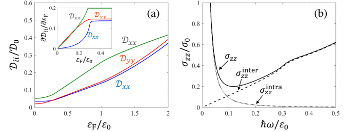
FIG. 5. (a) The Drude weight of tilted NLSMs with \Delta_t = 0.3\varepsilon_0 and (b) the intraband ( \sigma_{zz}^{\text{intra}} , dotted line) and interband ( \sigma_{zz}^{\text{inter}} , dashed line) contributions to the optical conductivity \sigma_{zz} (solid line). The inset to (a) shows the derivative of the Drude weight near \varepsilon_F = \Delta_t , where the Drude weight exhibits a nonanalytic kink behavior due to an abrupt change in the geometry of the FS. Here D_0 = \frac{e^2}{h}k_0\varepsilon_0 and the Drude weight is defined to be \sigma_{ii}^{\text{intra}} = D_{ii}\delta(\hbar\omega) . For (b), we use a finite broadening term \eta = 0.001\varepsilon_0 replacing the 0^+ term in Eq. (6) in SM.
