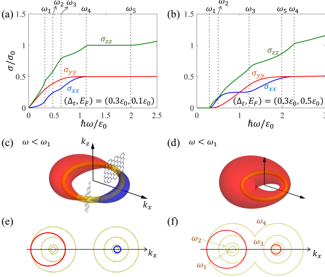
FIG. 4. (a), (b) Calculated optical conductivities of tilted NLSMs with \Delta_t = 0.3\varepsilon_0 for two different Fermi energies of (a) \varepsilon_F = 0.1\varepsilon_0 and (b) \varepsilon_F = 0.5\varepsilon_0 . (c), (d) The PS allowed by energy conservation indicated by a yellow torus along with electron (red) and hole (blue) pockets in the low frequency domain for (c) \varepsilon_F = 0.1\varepsilon_0 and (d) \varepsilon_F = 0.5\varepsilon_0 . (e), (f) Cross-sectional views of the electron-hole pockets and the PS allowed by energy conservation in the k_x - k_z plane at frequencies where kinks appear in the optical conductivity.
