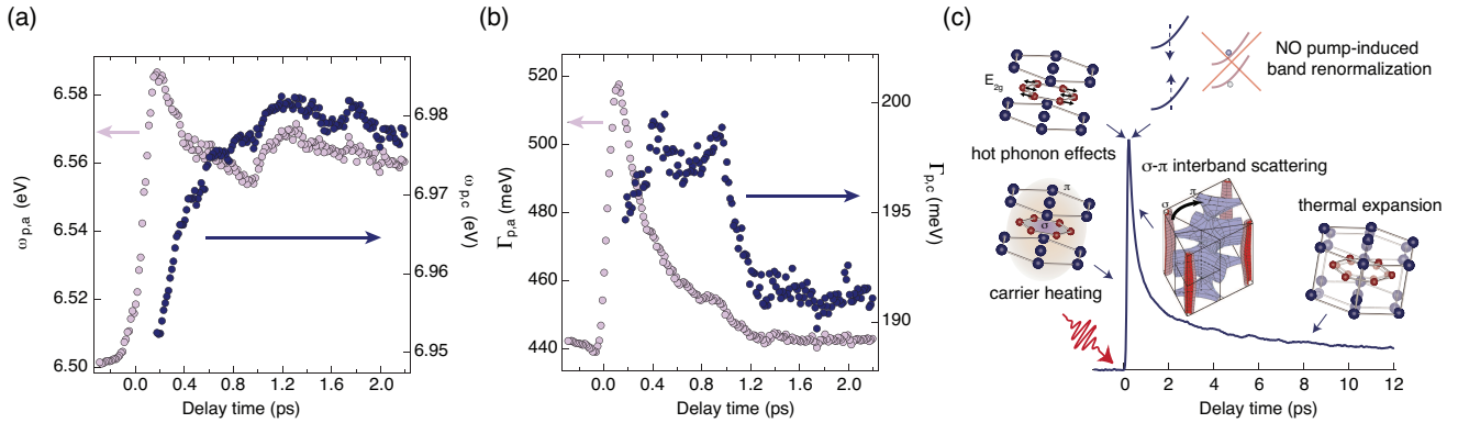
FIG. 3: Temporal evolution of (a) the bare plasma frequency \omega_{p,a/c} and (b) the optical scattering rate \Gamma_{a/c} along the a- (purple dots) and c-axis (blue dots). (c) Cartoon of the ultrafast dynamics. After the interaction with the solid, the ultrashort laser pulse leads to the excitation of both \sigma and \pi carriers. The nonthermal \sigma carriers are strongly coupled to the branch of the E_{2g} phonon mode and efficiently generate hot phonons during the first 170 fs. Subsequently the energy stored in the hot-phonon subsystem is released to the \pi carriers via interband scattering and to low-energy phonons via anharmonic decay.
