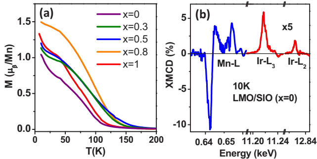
FIG. 1. Ferromagnetism in SLs. (a) Temperature dependence of magnetization for SLs. (b) XMCD spectra of SLs ( x=0 ) at both the Mn and Ir L_{2,3} edges measured under the same experimental conditions.
