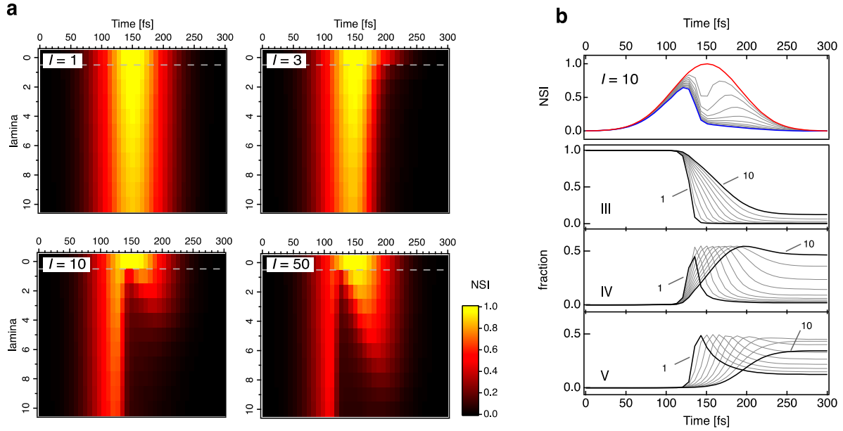
Figure 3. (a) Temporal evolution of the spectral intensity (SI) of the resonant x-ray photons through each lamina. Lamina “0” above the dashed line represents the incident x-ray pulse. The SI is normalized to the peak value of each incident pulse. (b) For the case of 1 \times 10^{17} W/cm 2 , the top panel shows the SI through each lamina, and the second to fourth panels display the temporal evolution of the charge state (CS) III ~ V at each lamina. The first (1) and the last (10) laminae are plotted with thick solid lines.
