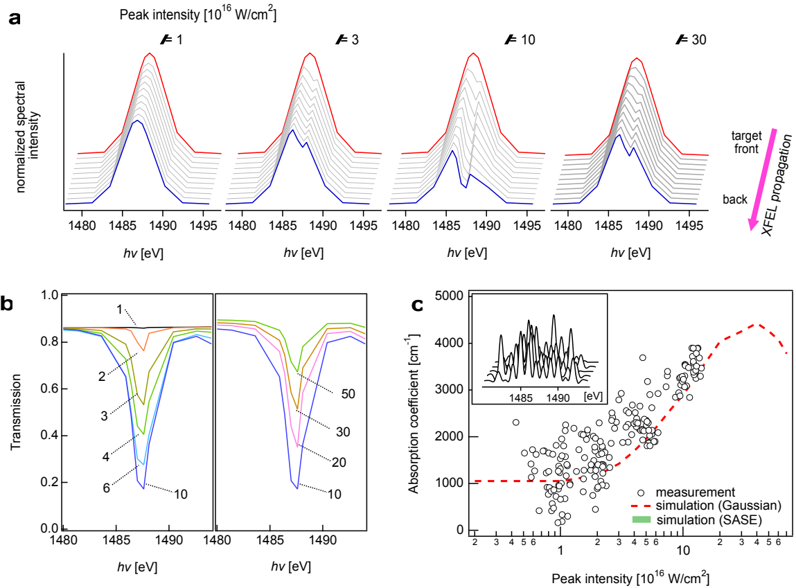
Figure 2. a) Simulation of transmitted x-ray spectra through an aluminum sample at selected intensities ( 1, 3, 10, 30 \times 10^{16} \text{ W/cm}^2 ). The incident and final transmitted spectra are depicted in the red and blue curves. The sample is divided into 10 laminae, and the transmission after each lamina is shown in grey. Each curve is normalized to the highest spectral intensity of the incident spectrum. (b) Final transmission spectra, obtained by the blue divided by the red curves in a), for I = 1 - 50 \times 10^{16} \text{ W/cm}^2 . (c) Absorption coefficient of aluminum as a function of peak intensity. The circles represent the experimental data at 1485 \sim 1490 \text{ eV} . The dashed line is the theoretical prediction from SCFLY. Note the intensity in (a) and (b) is at a single value without considering the intensity distribution of the XFEL focal spot. But in (c), the calculation includes the intensity distribution of the focal spot. [inset] Some simulation of transmitted SASE spectra. The incident spectra are corresponding to Gaussian profiles of 100 fs and 5 eV FWHM and a peak intensity of \sim 1 \times 10^{17} \text{ W/cm}^2 . In the main plot, the range of calculated absorption of 100 SASE pulse is shown as a green box.
