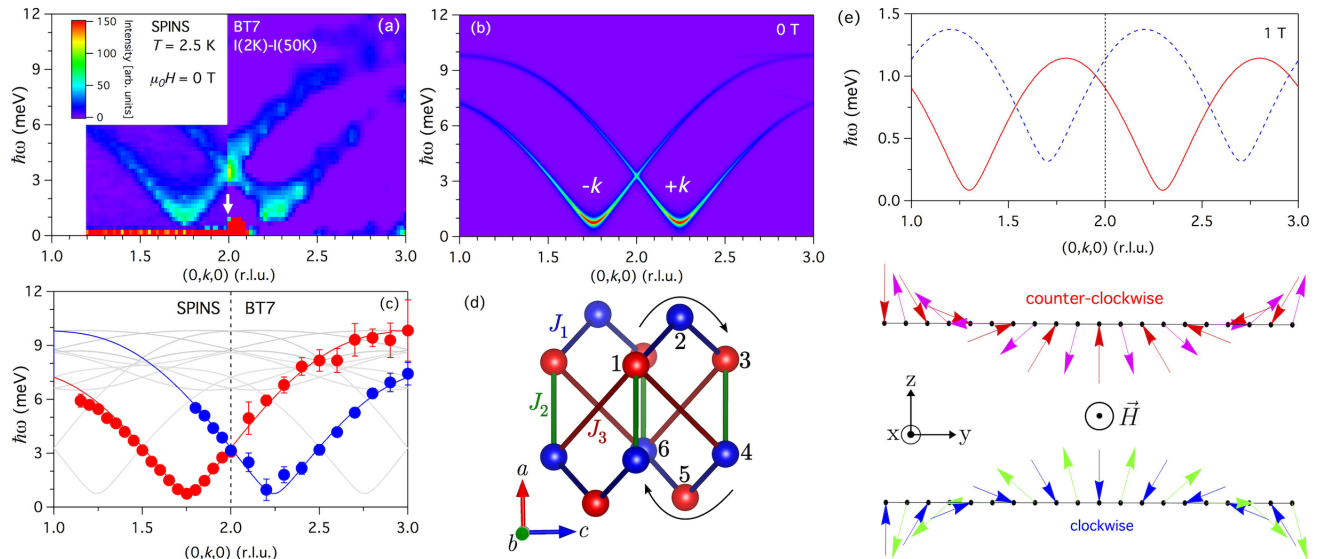
FIG. 1. (Color online) (a)–(c) The zero-field magnetic excitations in \alpha - \text{Cu}_2\text{V}_2\text{O}_7 . (a) The contour map, which is constructed from a series of constant- \mathbf{Q} scans taken at SPINS for k < 2 and at BT7 for k > 2 , shows two dispersive branches of the excitations centered around (0, 1.75, 0) and (0, 2.25, 0) . The BT7 contour map represents the intensity difference between the data measured at 2 K and 50 K. An arrow denotes the magnetic Bragg reflection at (0, 2, 0) . (b) The contour map of the calculated dynamical structure factor S(\mathbf{Q}, \hbar\omega) representing the spin-wave intensity along (0, k, 0) was calculated using the obtained fit parameters. (c) The spin-wave dispersions of all 16 branches are shown in grey, while red and blue lines represent the most intense branches. The data points were obtained from resolution-convolution fitting of the constant- \mathbf{Q} scans. Error bars denote standard derivations throughout the article. (d) The spin network of \alpha - \text{Cu}_2\text{V}_2\text{O}_7 is formed by three dominant exchange interactions J_1 , J_2 and J_3 . Red and blue spheres represent two spin sublattices, which are parallel and antiparallel to the a -axis, respectively. Arrows and spin labels denote the order of the cross product. (e) The magnetic excitations of the spin-chain model in an applied magnetic field along the x -axis (Eq. S1) were calculated with S = 1/2 , J = 1 meV, G = 0.26 meV, D = 1.0 meV, and H = 1 T (Supplementary Materials). Dynamical spin structures, which show the counterclockwise and clockwise rotation of the fluctuating spins around the field direction ( +x -direction), correspond to the solid red and dashed blue modes, respectively.
