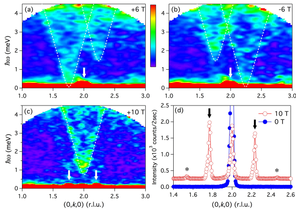
FIG. 2. (Color online) Spin-wave excitations in a magnetic field at 1.5 K. (a–c) show the energy-momentum contour maps measured at 6, -6 , and 10 T, respectively. Dashed lines denote the most intense branches resulting from the spin-wave calculations. (d) shows the magnetic Bragg peak measured along (0, k, 0) below and above the spin-flop transition (similar data measured at different fields are reported in Ref. 21). Arrows denote the magnetic Bragg peaks, and asterisks (*) indicate the second harmonic reflections.
