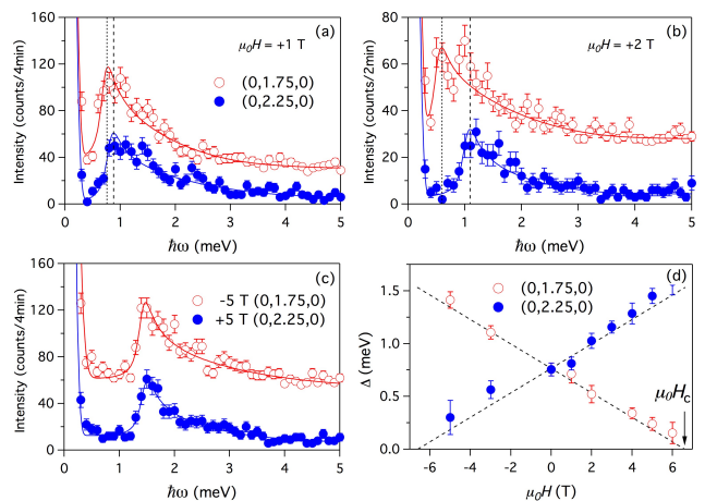
FIG. 3. (Color online) Constant- \mathbf{Q} scans were measured at (0, 1.75, 0) and (0, 2.25, 0) at (a) 1 T and (b) 2 T. The dashed and dotted lines denote positions of the energy gap. In (c), the scan at (0, 1.75, 0) and -5 T is compared with that at (0, 2.25, 0) and +5 T, which shows the same shift in energy. All (0, 1.75, 0) data are shifted for clarity. The gap energy as a function of field at (0, 1.75, 0) and (0, 2.25, 0) is shown in (d). The critical field is labelled by \mu_0 H_c , at which the energy gap vanishes.
