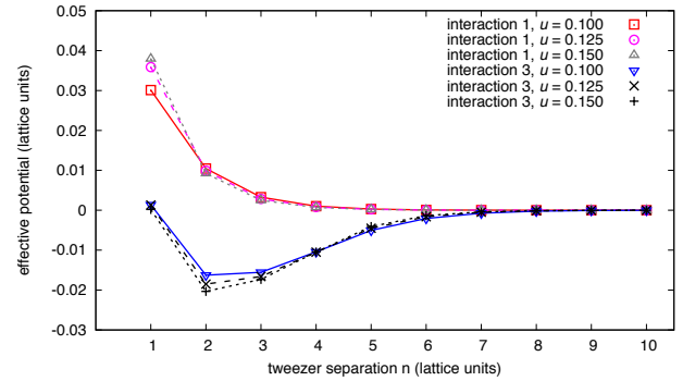
FIG. 2: The tweezer effective potential versus separation distance for interactions 1 and 3 for dimer binding energy 1/40 and tweezer couplings u = 0.100, 0.125, 0.150 .
