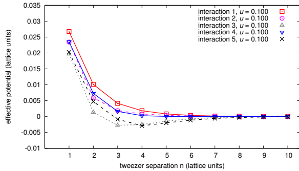
FIG. 5: The tweezer effective potential versus separation distance for interactions 1, 2, 3, 4, 5, with dimer binding energy 1/100 and tweezer coupling u = 0.100 .
