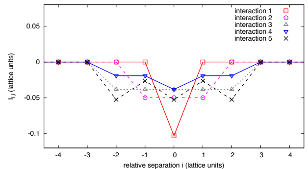
FIG. 4: Local part of the particle-particle interaction I_{i,i} versus relative particle separation i for interactions 1, 2, 3, 4, 5 and dimer binding energy 1/40 .
