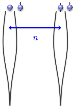
FIG. 1: Illustration of the external potential acting as numerical tweezers by holding the down-spin particles at separation distance n .
