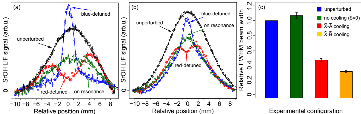
Figure 3. Integrated molecular beam profiles for different detunings of the cooling laser: (a) \tilde{X}(000) - \tilde{B}(000) and (b) \tilde{X}(000) - \tilde{A}(000) . The detunings from resonance are given by \delta = \pm 10 MHz. With a positive detuning, the width of the molecular beam is reduced, which indicates cooling of the molecular beam. A “hole” around zero for \delta < 0 represents a heating signature of the magnetically-assisted Sisyphus effect with the widening of the total spatial distribution. An asymmetry in the height of two peaks comes from imperfect alignment between laser and molecular beams and was previously seen in similar experiments with atoms [49]. The excess signal above the fit near zero position for the on-resonance trace in (b) is potentially indicative of a slightly positive detuning of the cooling lasers. (c) Summary of the cooling results in terms of the FWHM of the molecular cloud in the y dimension relative to the unperturbed distribution (no cooling lasers). Without cooling ( \delta = 0 ) the molecular beam profile is not modified significantly.
