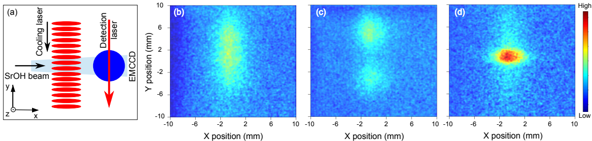
Figure 2. Spatial images of the molecular beam taken at different detunings of the \tilde{X}(000) - \tilde{B}(000) cooling laser: (b) on resonance, (c) red-detuned (-10 MHz), and (d) blue-detuned (+10 MHz). SrOH beam is moving in the x direction while the cooling and detection lasers are applied in the y direction as shown in (a). Narrowing of the spatial size of the molecular cloud with accompanying density increase in (d) compared to (b) in the y dimension indicates phase space compression.
