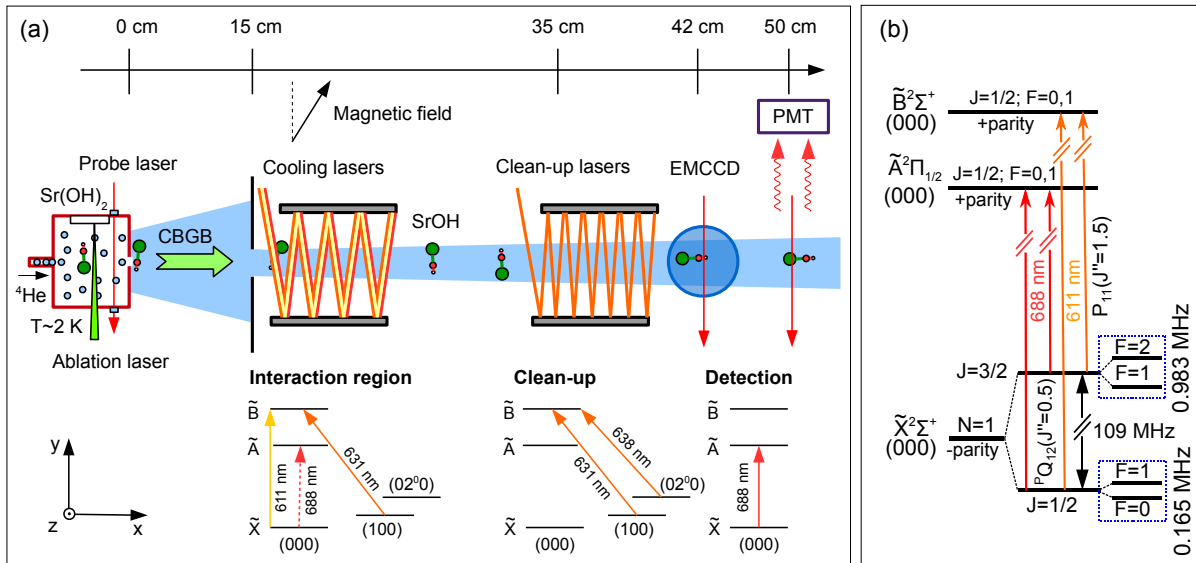
Figure 1. (a) Schematic of the experimental apparatus (not to scale). A cryogenic beam of SrOH is produced using laser ablation of \text{Sr}(\text{OH})_2 followed by buffer-gas cooling with \sim 2 K helium gas. To apply the cooling forces on the collimated molecular beam, we use transverse lasers retroreflected between two mirrors in order to generate a standing wave. Depending on the experimental configuration, either the \tilde{X}^2\Sigma^+(000) \rightarrow \tilde{A}^2\Pi_{1/2}(000) or the \tilde{X}^2\Sigma^+(000) \rightarrow \tilde{B}^2\Sigma^+(000) cooling transition is used with an additional \tilde{X}^2\Sigma^+(100) \rightarrow \tilde{B}^2\Sigma^+(000) laser for repumping molecules decaying to the vibrationally excited Sr-O stretching mode. In order to remix dark magnetic sub-levels, a magnetic field is applied at an angle relative to laser polarization in the Interaction region. Before the detection is performed, molecules remaining in either (100) or (02^0_0) excited vibrational levels of the electronic ground state are optically pumped back into the ground vibrational level using \tilde{X} \rightarrow \tilde{B} off-diagonal excitations. The spatial profile of the molecular beam is imaged on the electron multiplying charge-coupled device (EMCCD) camera and the time-of-flight (ToF) data is collected on the photomultiplier tube (PMT). The vibrational quantum numbers (v_1 v_2 v_3) correspond to the Sr \rightarrow OH stretching ( v_1 ), Sr-O-H bending ( v_2 ), and SrO \leftrightarrow H stretching ( v_3 ) vibrational modes. The superscript l next to the bending mode vibrational quantum number indicates the projection of the vibrational angular momentum on the internuclear axis. (b) Relevant rotational, fine, and hyperfine structure of SrOH. Rotationally closed excitations on the \tilde{X} - \tilde{A} and \tilde{X} - \tilde{B} electronic transition are shown with red and orange upward arrows, correspondingly. The unresolved hyperfine splittings have been previously measured [59] and are smaller than the natural linewidth of the electronic transitions [60].
