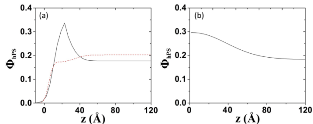
FIG. 1 (a) Experimentally measured hPS segment volume fraction depth profiles for the 37k cyclic/linear (solid curve) and 37k linear/linear (dashed curve) blend films after annealing at 180 °C for 12 h. (b) Segment volume fraction depth profile for a 37k cyclic/linear blend with ideally smooth surface calculated using SCFT, with \chi_{\text{cyclic}}=0.2 , total bulk segment density \rho_b=1.0 , b=6\text{\AA} , and v=1b^3 .
