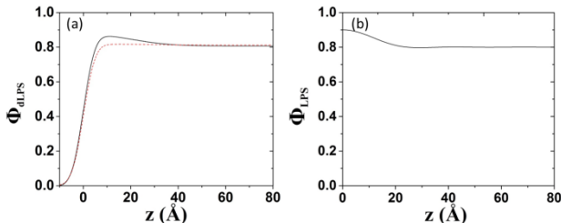
FIG. 2 (a) Comparison of linear dPS segment volume fraction depth profiles from NR for the 2k cyclic/linear blend film (solid curve) and 2k linear/linear blend film (dashed curve) after annealing at 120 °C for 12h. (b) Smoothed segment volume fraction profile for the 2k cyclic/linear blend with ideally smooth surface calculated using Wall-PRISM with \chi_{\text{cyclic}}=0.2 , N=20 beads, total bulk segment density \rho_b = 1.0 , packing fraction of 0.45, and 80/20 ratio of linear to cyclic polymers.
