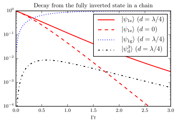
FIG. 4. Decay of three \Lambda -type atoms in an equidistant chain of distance d = \lambda/4 with non-equal \Gamma_j^{ik} starting from the totally inverted state |eee\rangle . The solid red line gives the excited state population per atom, the dotted blue line shows the population in the ground state subspace and the dashed-dotted black line gives the dark state |\psi_d^3\rangle fraction during the decay. For comparison the red dashed line exhibits ideal collective decay at d = 0 with all equal \Gamma_j^{ik} (Dicke case). Note, that during the evolution the dark (gray) state, which decays much slower, becomes populated partially. Again, we neglect \Omega_j^{ik} , which would lead to an oscillatory behavior in the populations.
