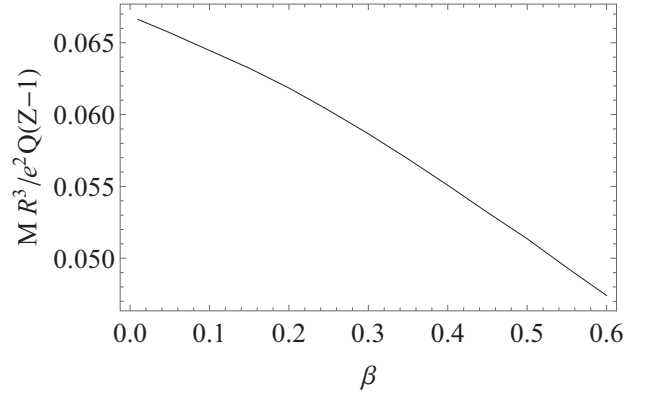
FIG. 1: Dependence of the ratio M/Q on the nuclear quadrupole deformation size \beta .
