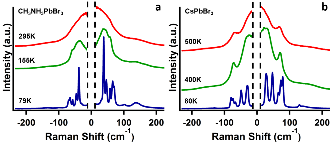
FIG. 1. Low-frequency Raman spectra of hybrid and inorganic lead-halide perovskite crystals. The spectral region obscured by the notch-filter, between \pm 10 \text{ cm}^{-1} (marked by the vertical dashed lines), has been deleted. (a) \text{CH}_3\text{NH}_3\text{PbBr}_3 and (b) \text{CsPbBr}_3 in the orthorhombic phase (blue), tetragonal phase (green), and cubic phase (red), showing growth of central peak with temperature in both materials.
