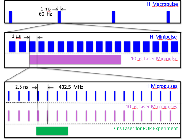
FIG. 2. The macropulse (top), minipulse (middle) and micropulse (bottom) structure of the \text{H}^- beam (blue), the laser in this 10 \mu\text{s} experiment (light purple), and the laser in the POP experiment (green).
