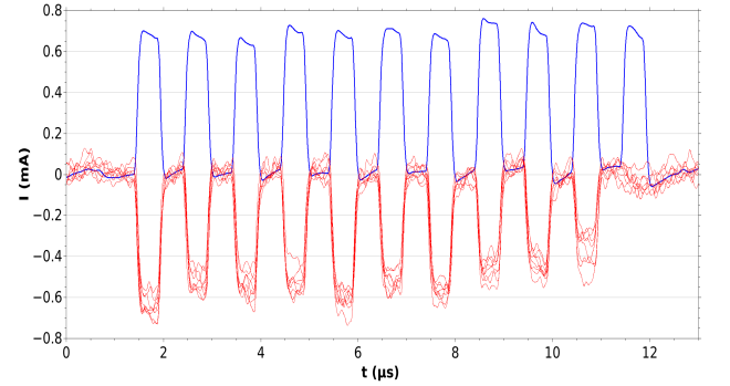
FIG. 4. The experimental results. The average beam current for a 11 \mu s H^- beam measured by the beam current monitor at the interaction point before stripping (blue), and eight separately measured stripped proton beam pulses on the same beam current monitor during stripping (red).
