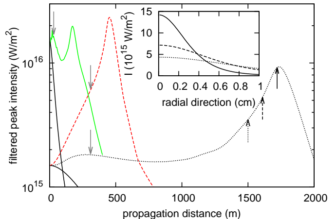
FIG. 4. Spectrally filtered peak intensity versus propagation distance for different 10 \mu\text{m} LWIR USPs. The green curve is for a 2.4 TW USP of 240 fs duration and 1.2 cm wide (same as in Fig. 3), the red-dashed curve is for 240 fs and 3.7 cm, and the black-dotted curve is for 1.2 ps and 3.7 cm. The gray arrows indicate the Rayleigh ranges of 31 m and 310 m respectively, while the black solid curves indicate the intensities for linearly propagating beams. The inset shows the unfiltered radial intensity of the 1.2 ps USP at the positions indicated by the black arrows with matching line style. The initially 3.7 cm wide pulse collapses down to 0.6 cm.
