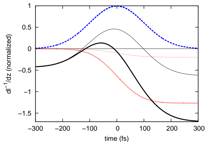
FIG. 2. Kerr lensing (blue-dashed curve) and dynamic plasma lensing (red-dotted curves) contributions as functions of time delay with respect to the pulse center, see Sec. III of the SI. The black curves show the net lensing experienced by the pulse including diffraction. Results are for a 10 \mu\text{m} (wide lines) and 4 \mu\text{m} (thin lines, parameters in brackets if different) USP of beam width 1.2 (0.48) cm, length 240 fs, peak intensity 1.5 \times 10^{16} \text{ W/m}^2 , corresponding to a peak power of 2.4 (0.38) TW equivalent to 1.6 critical powers, and a pulse energy of 590 (94) mJ. The values are scaled to the maximum of the Kerr contribution for each pulse respectively.
