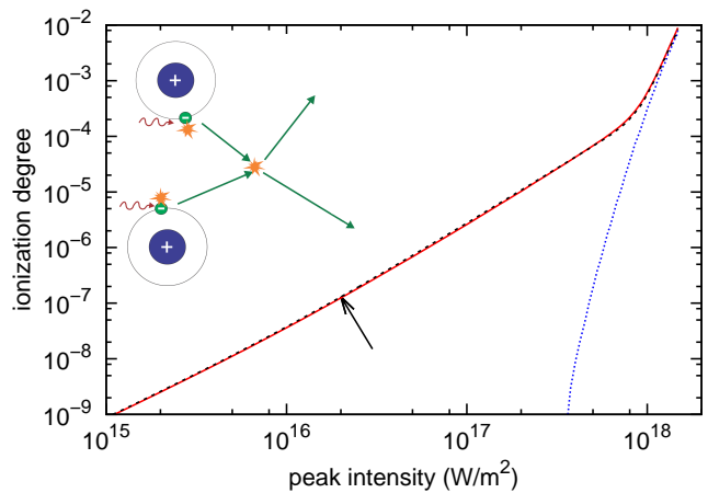
FIG. 1. Ionization degree versus peak intensity for a 200 fs LWIR USP at 10 \mu\text{m} . The blue-dotted curve shows the ionization degree based on single-atom ionization, the red curve shows the results from the full microscopic theory, and the dashed black curve shows the results from the rate equation model supplemented by the single-atom ionization. Here the optimized fit parameters c = 3.04 \cdot 10^{-7} \frac{1}{\text{m}^3 \text{s}} \frac{\text{m}^4}{\text{V}^4} and s = 4.6 \cdot 10^{18} \frac{\text{V}^2}{\text{m}^2} were employed for argon at 1 atm. The arrow indicates the peak intensity reached in our propagation simulations, and this remains well below the threshold value 2 \times 10^{17} \text{ W/m}^2 for single-atom ionization. The inset illustrates that the many-body interaction involves electrons from different atoms.
