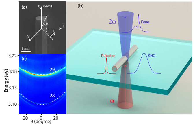
FIG. 1. (a) The scanning electron image (SEM) of a typical ZnO microwire. The angles defined as \theta and \phi represent the two detection planes of the angle resolved spectra. (b) The fundamental light wave irradiates the ZnO microwire from back of the glass, the SHG radiation is emitted from the top of the wire. (c) The dispersion of the 28 th and 29 th TM polarized polariton modes, fitting with the white dashed lines.
