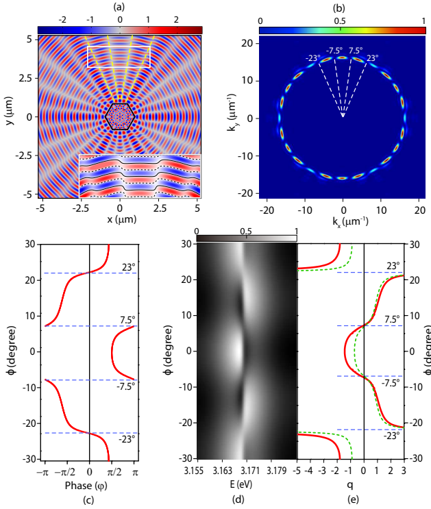
FIG. 4. (a): The electric field distribution pattern for the 29 th polariton mode in the real space calculated using finite element analysis. Inset: the equiphase surface marked by the dashed and solid lines for the white rectangle area. (b): The Fourier Transform of pattern (a). The dashed lines marked the angles where the phase of the emission electric field in pattern (a) change sign. (c): The phase \varphi v.s. \phi curve obtained with use the phase information in (a). (d): The theoretical pattern calculated by using equation (3) with A_p/\Gamma_p being the amplitude against \phi obtained from (b) and A_s/\Gamma_s being the same order of A_p/\Gamma_p . \Gamma_p and \Gamma_s are the FWHM (in frequency domain) of the 29 th polariton mode (1.3 meV) and SHG (12 meV) respectively. (e): The q variation obtained by fitting each line of pattern d (red solid line) and q(\varphi)=-\cot(\varphi/2) (green dashed line).
