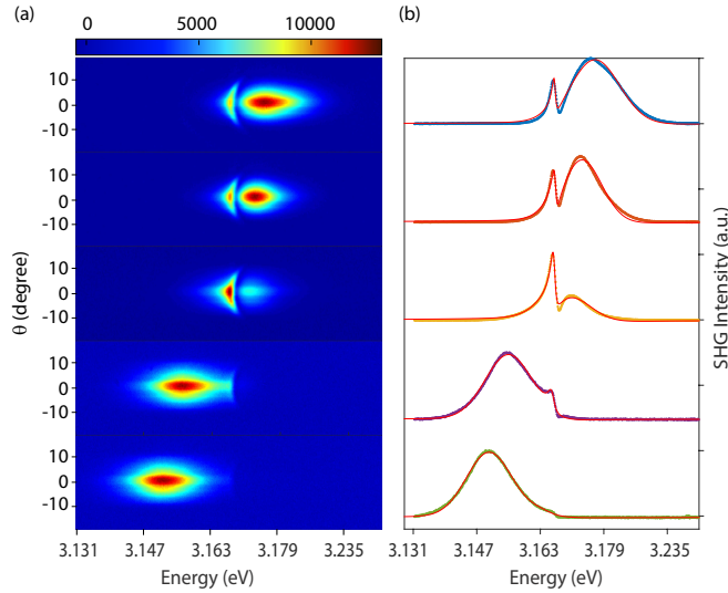
FIG. 2. (a): Angle \theta resolved SHG spectra with the peak at 3.175 eV, 3.172 eV, 3.169 eV, 3.155 eV, 3.151 eV from up to down. (b): the corresponding line curves at \theta=0^\circ , fitting with the red solid lines by equation (1).
