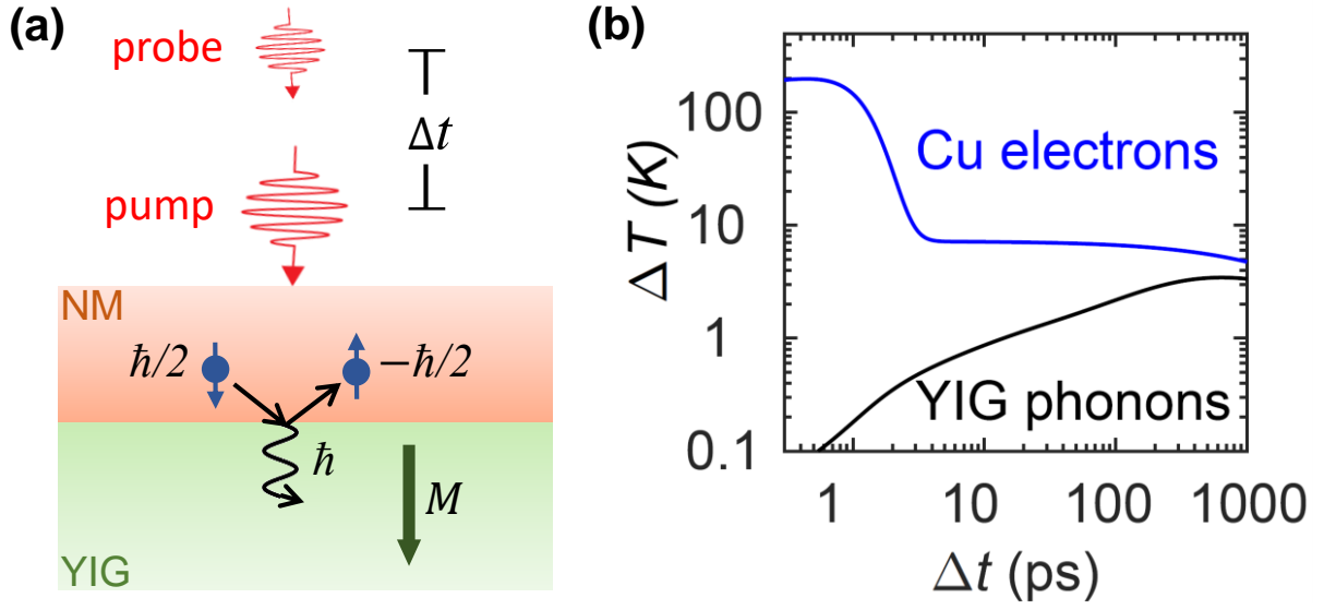
FIG. 1: (Color online). Conceptual diagram and temperature transients. (a) Absorption of a pump laser pulse of picosecond duration generates a temperature difference between NM electrons and YIG magnons. Interfacial coupling between electrons and magnons induces spin accumulation in NM, which is probed by time-delayed probe laser pulses. (b) Example temperature transients of Cu electrons and YIG phonons calculated using the 2TM, Eqs. (1) and (2).
