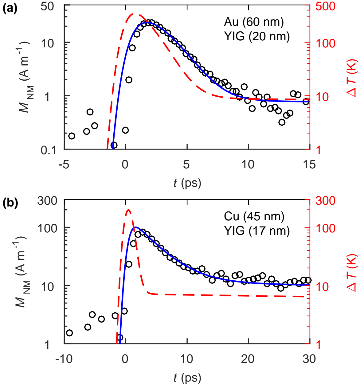
FIG. 2: (Color online). Thermally-induced spin accumulation in Au and Cu. TR-MOKE data (symbols) measured on Au (Cu)/YIG/GGG samples of different layer thicknesses stated in the figure. Solid lines show fit curves obtained using the spin-diffusion model, Eqs. (3) and (4). Dashed lines show temperature excursion of electrons calculated using the 2TM, Eqs. (1) and (2).
