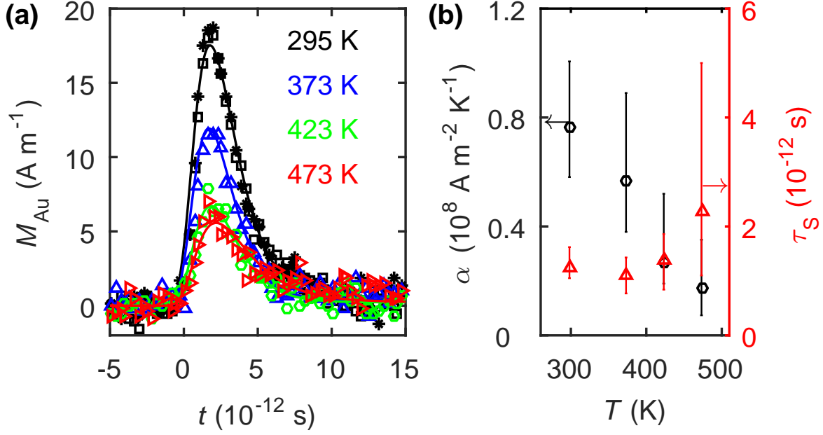
FIG. 3: Temperature-dependent measurements. (a) TR-MOKE data (symbols) measured on sample I at different temperatures as indicated. Solid lines show fit curves obtained using the spin-diffusion model. (b) Fit results for \alpha = g_{\uparrow\downarrow}e^2/hS_S (left y -axis) and spin relaxation time \tau_S (right y -axis) as function of temperature.
