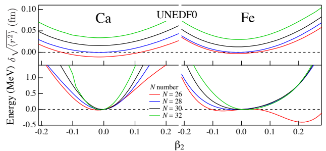
FIG. 3. rms charge radii (top) plotted relative to \sqrt{\langle r^2 \rangle} at N = 28; \beta_2 = 0 , and potential energies (bottom) for the Ca (left) and Fe (right) chains calculated with UNEDF0 as a function of \beta_2 . Results with SV-min (not shown) are similar.
