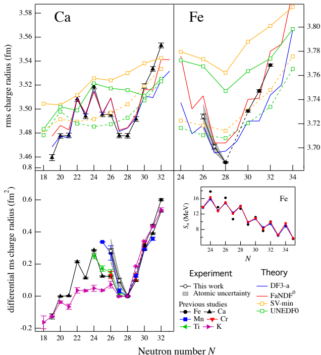
FIG. 2. rms charge radii (top) of the isotopic chains of Ca (left) and Fe (right), and differential rms charge radii (bottom) of K - Fe (left). Data are taken from Refs. [21, 22, 40, 49–51] and this work. The uncertainties in the atomic factors are marked by shading. Calculations with SV-min and UNEDF0 EDFs were performed for even-even mass isotopes only. The inset shows one-neutron separation energies for the Fe chain.
