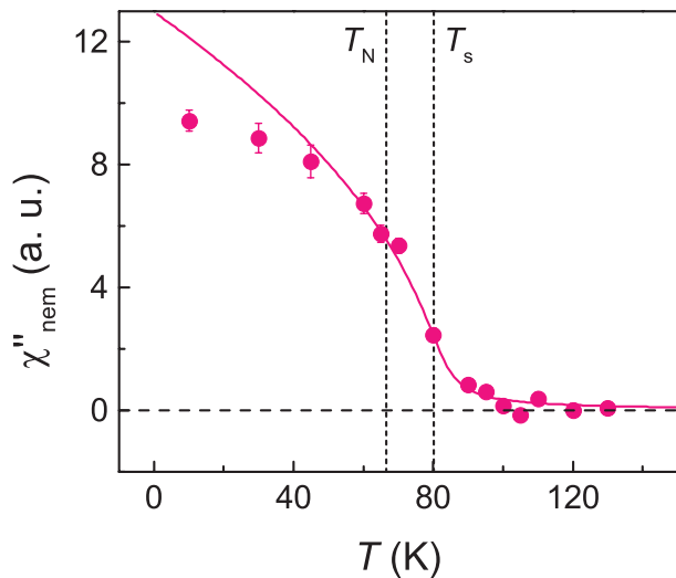
FIG. 4: Temperature dependence of \chi''_{nem} . The solid line is calculated according to the Landau free energy as described in the main text with a_0 = 3.73 , b = 0.036 and h = 266 . The vertical dashed lines indicate T_s and T_N .
