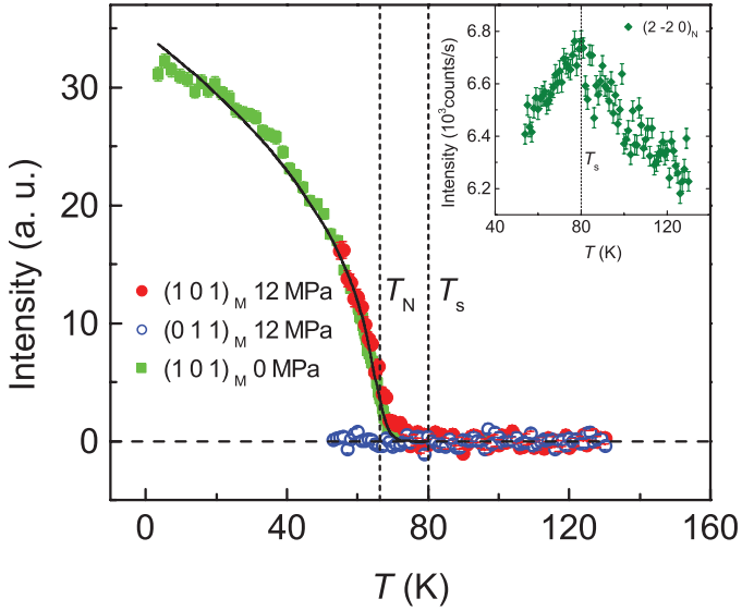
FIG. 1: Temperature dependence of the intensity of the AF Bragg peaks at (1 0 1) and (0 1 1) under 0 and 12 MPa. The solid line is fitted as described in the text. T_N is determined from the fitting. The inset shows the temperature dependence of the intensity of the nuclear Bragg peak at (2 -2 0), which shows a kink at T_s .
