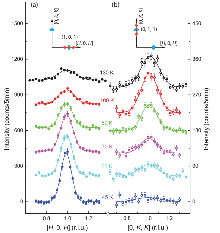
FIG. 2: Background-subtracted \mathbf{Q} -scans at 7 meV along (a) (H 0 H) and (b) (0 K K). The data are shifted for different temperatures. The solid lines are the Gaussian fits of the data.
