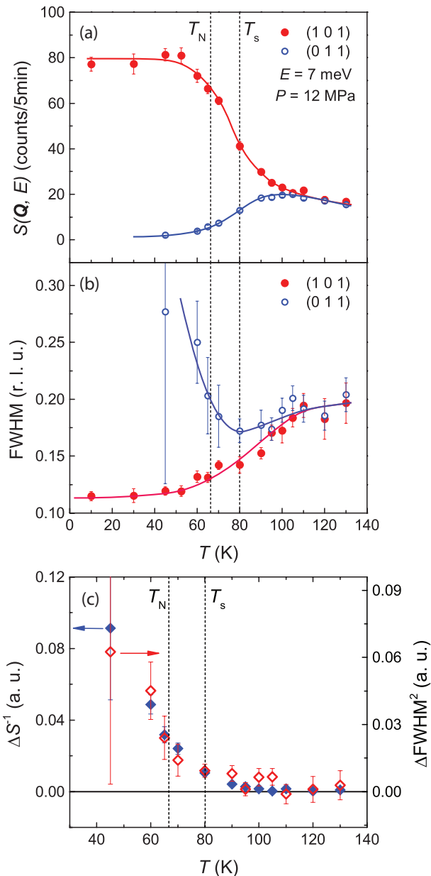
FIG. 3: Temperature dependence of (a) S(\mathbf{Q}, E) and (b) FWHM at (1 0 1) and (0 1 1) at 7 meV and 12 MPa. (c) Temperature dependence of \Delta S^{-1} (blue solid diamonds) and \Delta \text{FWHM}^2 (red open diamonds) as defined in the main text. The solid lines are guided to the eye. The vertical dashed lines indicate T_s and T_N . The error bars are given by the Gaussian fits.
