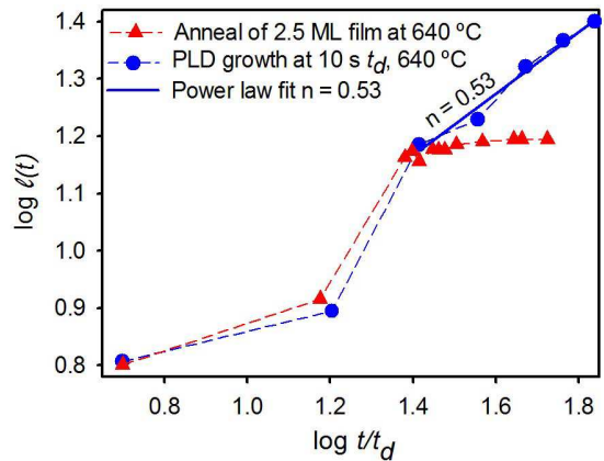
FIG. 4. Illustration of the negligible change of the correlation length (red triangles) for a \text{SrTiO}_3 film that was annealed at a substrate temperature of 640 °C after growth was stopped at the third diffuse scattering maximum ( \sim 2\frac{1}{2} ML) compared to the increasing correlation length in continuous film growth (blue dots). The complete data are shown in Fig. S2b.
