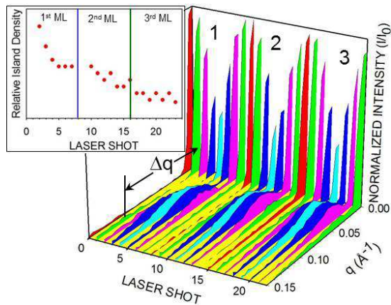
FIG. 1. 3D line plot of the SXR D intensities as a function of q for single laser shots of SrTiO 3 growth at 650 °C and 10 s dwell time that corresponds to the time between successive laser shots. The growth intensity oscillations for the growth of the first 3 MLs are shown on the back (vertical) plane, and the out of phase diffuse scattering oscillations are shown on the front (horizontal) plane. A ML corresponds to a unit cell consisting of one SrO/TiO 2 bilayer. The inset shows corresponding island densities extracted from the diffuse scattering data as N(t) \sim (\Delta q)^2 for the first 3 unit cell growth.
