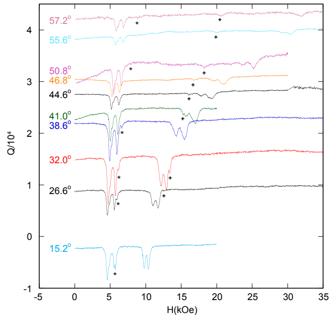
FIG. 2. Absorption ESR spectra at 1.8 K for several angles \theta_H . The spectrum for \theta_{H,ref} = 26.6^\circ shows actual Q values. All other spectra have been shifted vertically by an amount proportional to \theta_H - \theta_{H,ref} . Spectra from three different crystals are combined in this figure. Each spectrum has been shifted slightly horizontally to account for inductive effects due to sweeping H (see [28]).
