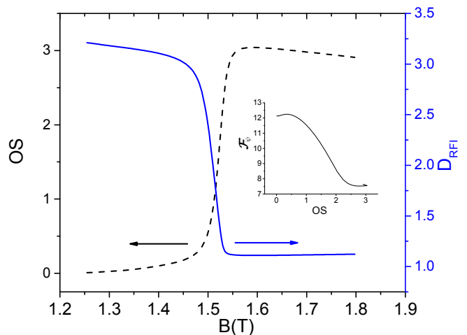
FIG. 5. Oscillator strength (OS) and D_{RFI} for one of the transitions studied as a function of field. Here |i\rangle \approx |m = 3\rangle and |f\rangle = |E_3\rangle are the second- and third-lowest energy eigenstates (cf. Fig. 1), respectively. As the field increases, the angle \theta is adjusted to maintain resonance of the transition with the radiation frequency. For this pair of levels, the transition is forbidden (allowed) at small (large) fields with a crossover at the field of the anticrossing. The inset shows a parametric plot of \mathcal{F}_\psi vs. OS, illustrating how, near the anticrossing, one quantity rises as the other falls, but both can be substantial over some region. Similar calculations for the transition between |E_2\rangle and |E_4\rangle , the second and fourth energy eigenstates, show complementary behavior [28].
