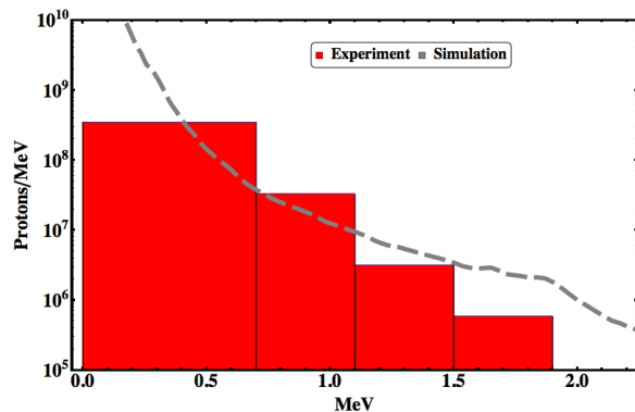
FIG. 6. Plot comparing experimental to simulated proton energy spectrum for n_e = 0.3 n_{CRIT} . Proton distribution asymmetries, simulated experimental parameters, or sampling statistics with PIC macroparticles may be the cause of discrepancies at higher energies.
