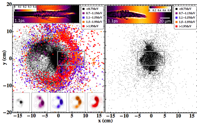
FIG. 4. The spatial distribution of test particles as projected to the plane of the detector for 0.3n_{crit} (left) and 0.6n_{crit} (right). The gray box indicated the region extracted in Fig. 3. Inset below are contour plots of the proton spatial distributions corresponding to the various energy buckets. Inset above are proton density plots taken along the polarization plane for each case. Note that for the 0.3n_{crit} case the cavitation region extends the entire length of the plasma while it only extend halfway through for the 0.6n_{crit} .
