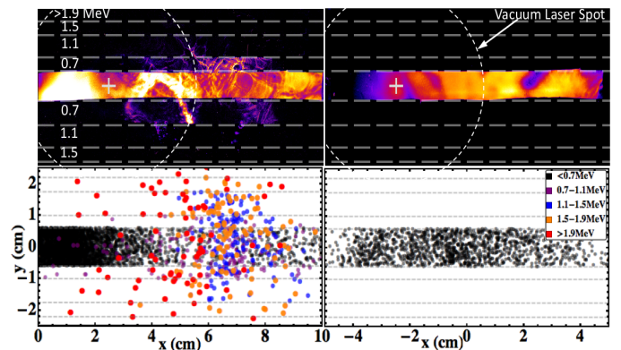
FIG. 3. False color image of 10cm x 5cm CR-39 plates for the cases of 0.3 n_{crit} (left) and 0.6 n_{crit} (right). The detector covers a solid angle of 0.25 sr. The laser axis and vacuum spot size are included on both. Dashed horizontal lines represent the location of the filters and their lower energy bound is listed on the left. On the bottom are plots of simulated test particles projected to the plane of the detector color-coded to the experimental energy buckets. See fig. 4 for contour plots of the simulated proton distribution.
