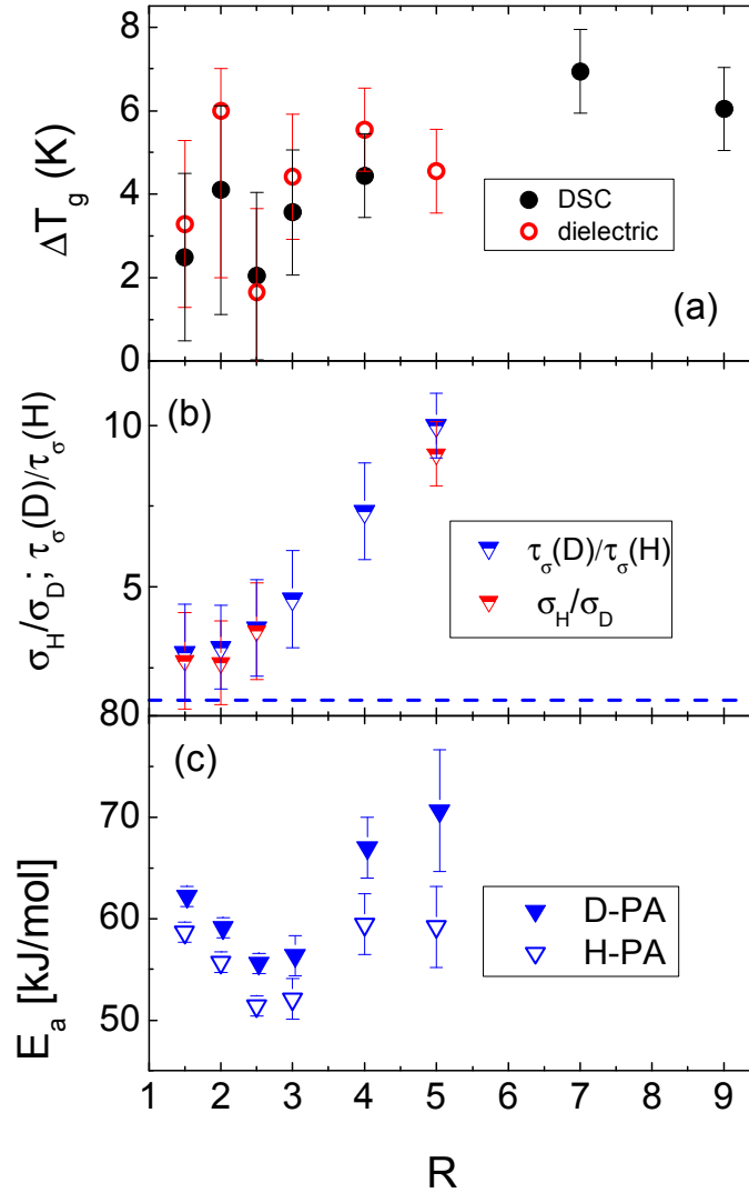
Figure 3. Dependence of the isotope effect on molar content of water R: (a) Isotope shift of the glass transition temperature \Delta T_g = T_g(D) - T_g(H) measured by DSC (closed symbols) and BDS (open symbols). The error-bars for the shift in T_g are larger for samples with low R due to significantly higher sensitivity of T_g in these samples to the water content. (b) The ratio of the conductivities and conductivity relaxation times at T_g . The dashed line shows the ratio \sigma_H/\sigma_D \sim 1.4 . (c) The activation energy for the conductivity relaxation time in the Arrhenius
