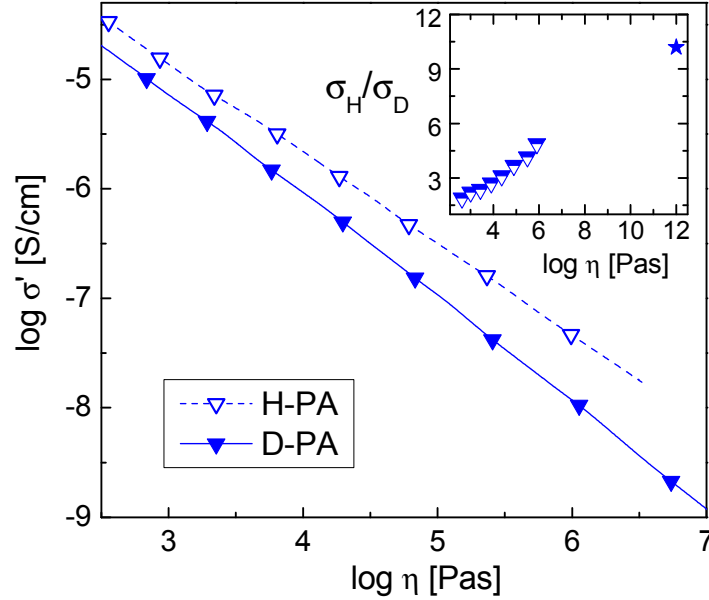
Figure 4. Conductivity vs. viscosity in protonated (open symbols) and deuterated (closed symbols) PA with R=5 . Inset shows the ratio of conductivities at the same viscosity that increases with decrease in temperature (increase in viscosity), and the star shows the ratio of conductivities at T_g that should correspond to \eta \sim 10^{12} Pa*s.
