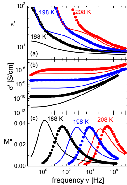
Figure 1. Dielectric spectra of R=3 H-PA (solid symbols) and D-PA (lines) at select temperatures. (a) Real part of the dielectric permittivity \epsilon'(\nu) ; (b) real part of the conductivity \sigma'(\nu) ; and (c) imaginary part of the electric modulus M''(\nu) .
