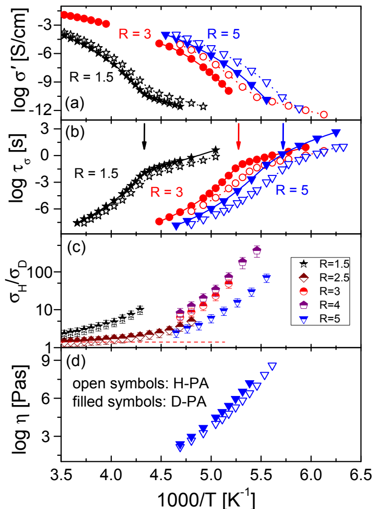
Figure 2: Temperature dependence of (a) conductivity, and (b) of the conductivity relaxation time in H-PAs (opened symbols) and in D-PAs (closed symbols) for several selected water content R values. Arrows in (b) indicate T_g values for H-PAs from DSC measurements. (c) The ratio of conductivities in protonated \sigma_H and deuterated \sigma_D samples with different R . The horizontal dashed line in (c) presents the value 1.4 expected for classical proton transfer mechanism. (d) Temperature dependence of viscosity in H-PA (open triangles) and D-PA (closed triangles) with R=5 .
