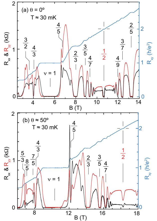
FIG. 2. (color online) Magneto-resistance traces for the sample of Fig. 1, measured at \theta = 0^\circ and 50^\circ . Both R_{xx} and R_{yy} are much smaller near \nu = 1/2 than in Fig. 1(e) data.
