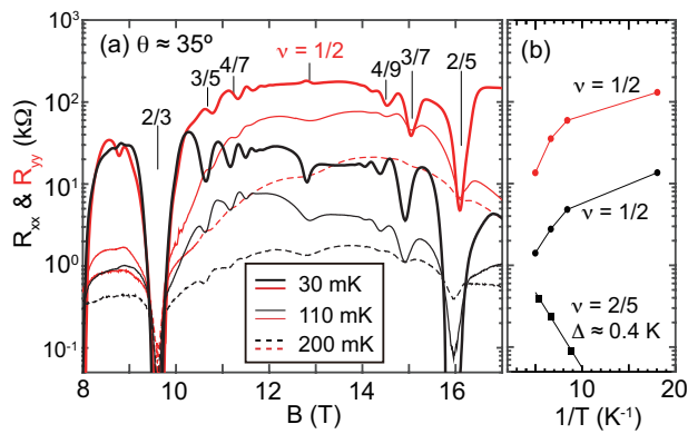
FIG. 3. (color online) (a) R_{xx} and R_{yy} measured at three temperatures in the 40-nm-wide QW near \nu = 1/2 at \theta \simeq 35^\circ . (b) T -dependence of R_{xx} and R_{yy} near \nu = 1/2 . To avoid the influence of the relatively sharp \nu = 1/2 resistance minima seen in some of the traces, here we are plotting the background resistances by interpolating between the shoulders flanking the \nu = 1/2 minima. Also plotted is the T -dependence of the R_{xx} minimum for the \nu = 2/5 FQHS.
