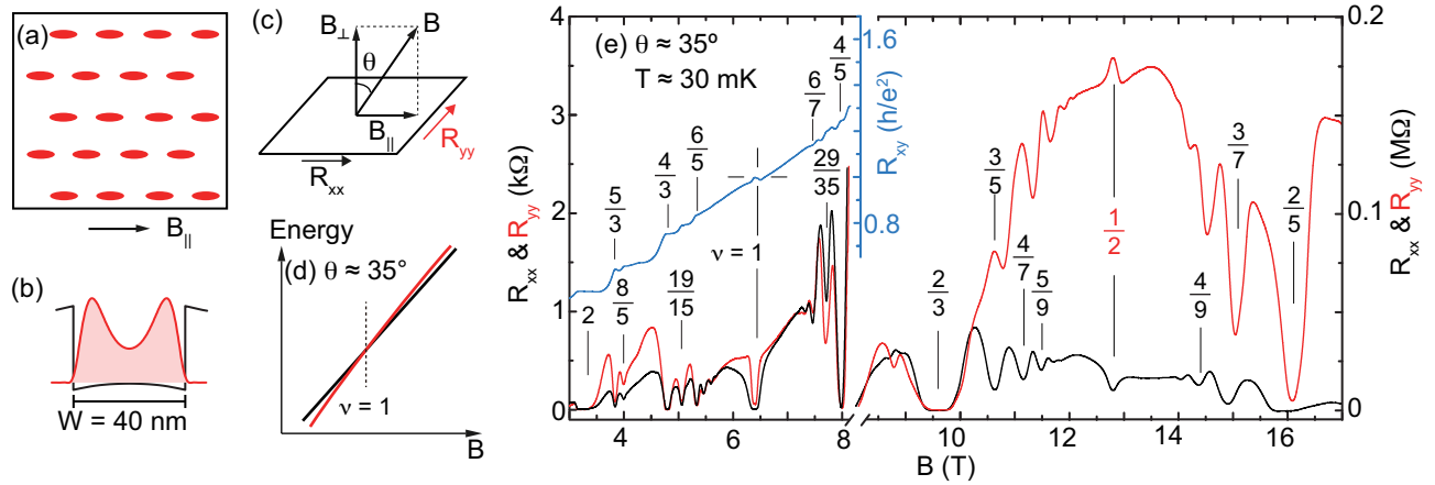
FIG. 1. (color online) (a) Conceptual rendition of an anisotropic (striped) Wigner crystal. (b) The charge distribution (red) and potential (black), from calculating the Schroedinger and Poisson's equations self-consistently at B = 0 . (c) Experimental geometry: R_{xx} and R_{yy} denote the longitudinal magneto-resistance measured along and perpendicular to the parallel magnetic field ( B_{\parallel} ), respectively. (d) Schematic diagram, showing the crossing of the lowest two Landau levels at \theta \simeq 35^\circ near \nu = 1 . (e) Magneto-resistance traces measured at tilt angle \theta \simeq 35^\circ for a 2DHS with density p = 1.28 \times 10^{11} \text{ cm}^{-2} and confined to a 40-nm-wide GaAs QW. Note the factor of 50 change in the scale for R_{xx} and R_{yy} for B > 8 \text{ T} . We observe an anisotropic insulating phase in a large filling factor range, from \sim 2/3 to \sim 1/3 ; note also the competition with FQHSs at several fillings.
