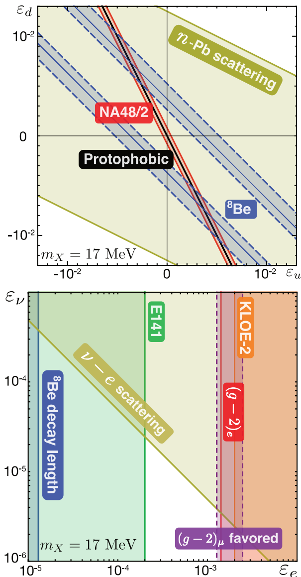
FIG. 1. The required charges to explain the {}^8\text{Be} anomaly in the (\varepsilon_u, \varepsilon_d) (top) and (\varepsilon_e, \varepsilon_\nu) (bottom) planes, along with the leading constraints discussed in the text. Top : The n -Pb and NA48/2 constraints are satisfied in the shaded regions. On the protophobic contour, \varepsilon_d/\varepsilon_u = -2 . The width of the {}^8\text{Be} bands corresponds to requiring the signal strength to be within a factor of 2 of the best fit. Bottom : The E141, KLOE-2, (g-2)_e , and \nu - e scattering constraints exclude their shaded regions, whereas (g-2)_\mu favors its shaded region. The {}^8\text{Be} signal imposes a lower bound on |\varepsilon_e| .
