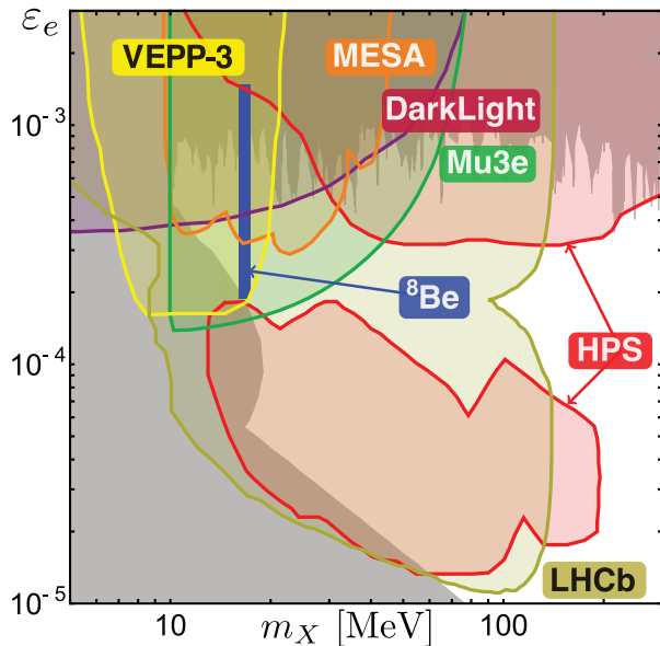
FIG. 2. The {}^8\text{Be} signal region, along with current constraints discussed in the text (gray) and projected sensitivities of future experiments in the (m_X, \varepsilon_e) plane. For the {}^8\text{Be} signal, the other couplings are assumed to be in the ranges given in Eq. (10); for all other contours, the other couplings are those of a dark photon.
