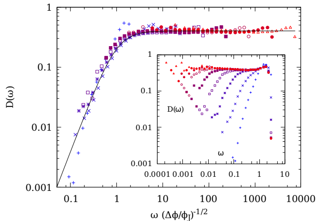
Figure 1. DOS for a single configuration in d = 4 for N = 8192 with rescaled \omega . The collapsed data is fitted to Eq. (3) (solid line). Inset: DOS for \Delta\phi/\phi_J = 9.1 \times 10^{-8}, 9.2 \times 10^{-7}, 9.2 \times 10^{-6}, 9.2 \times 10^{-5}, 9.0 \times 10^{-4}, 8.7 \times 10^{-3}, 8.0 \times 10^{-2} and 9.4 \times 10^{-1} , from left to right. Errors are smaller than the symbol size, except at very low \omega , where they are comparable to the data scatter.
