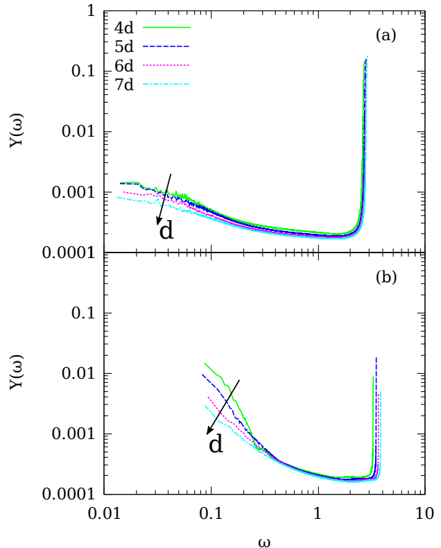
Figure 4. IPR for N = 8192 particles in d = 4-7 , averaged over 30 to 50 configurations, (a) moderately compressed \Delta\phi/\phi_J \approx 0.2 and (b) highly compressed \Delta\phi/\phi_J \approx 1.4 above jamming. Statistical errors are comparable to the data scatter.
