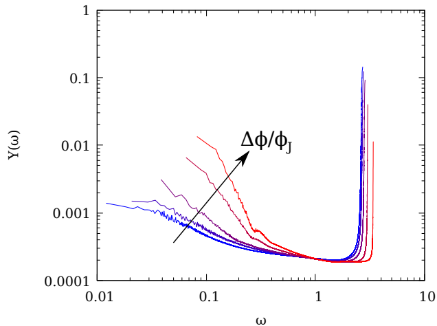
Figure 3. Evolution of IPR with frequency in d = 4 for N = 8192 averaged over 50 configurations for \Delta\phi/\phi_J = 1.5 \times 10^{-2} , 4.7 \times 10^{-2} , 1.5 \times 10^{-1} , 5.1 \times 10^{-1} and 1.6. Statistical errors are comparable to the data scatter.
