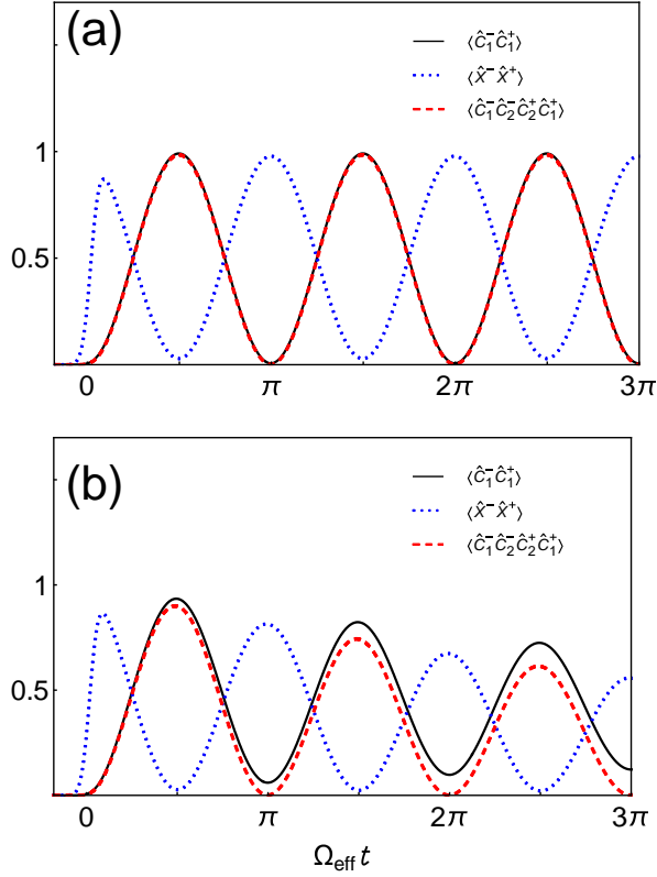
FIG. 3. (Color online) (a) Time evolution of the cavity mean photon number \langle \hat{X}^- \hat{X}^+ \rangle (dotted blue curve), qubit 1 mean excitation number \langle \hat{C}_1^- \hat{C}_1^+ \rangle (continuous black curve), and the zero-delay two-qubit correlation function G_q^{(2)} = \langle \hat{C}_1^- \hat{C}_2^- \hat{C}_2^+ \hat{C}_1^+ \rangle (dashed red curve) after the arrival of a \pi -like Gaussian pulse initially exciting the resonator. After the arrival of the pulse, the system undergoes vacuum Rabi oscillations showing the reversible joint absorption and re-emission of one photon by two qubits. \langle \hat{C}_1^- \hat{C}_1^+ \rangle and G_q^{(2)}(t) are almost coincident. This perfect two-qubit correlation is a signature that the two qubits are jointly excited. (b) Time evolution of the cavity mean photon number (dotted blue curve), the qubit mean excitation number, and the two-qubit correlation as in (a), but including the effect of cavity damping and atomic decay. The corresponding rates are \kappa = \gamma = 4 \times 10^{-5} \omega_q .
