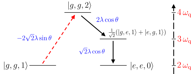
FIG. 1. (Color online) Sketch of the process giving the main contribution to the effective coupling between the bare states |g, g, 1\rangle and |e, e, 0\rangle , via intermediate virtual transitions. Here, the excitation-number nonconserving processes are represented by arrowed dashed line. The transition matrix elements are also shown.
