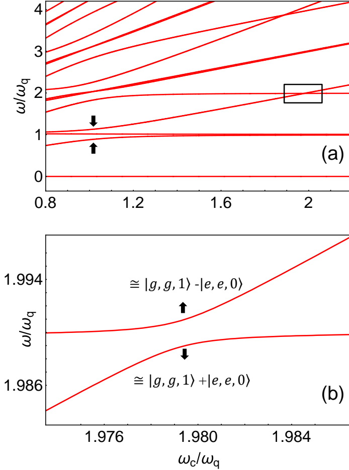
FIG. 2. (Color online) (a) Frequency differences \omega_{i,0} = \omega_i - \omega_0 for the lowest energy eigenstates of Hamiltonian (1) as a function of \omega_c/\omega_q . Here we consider a normalized coupling rate \lambda/\omega_q = 0.1 between the resonator and each of the qubits. We used \theta = \pi/6 . The black arrows indicate the ordinary vacuum splitting arising from the coupling between the states |g, g, 1\rangle and (1/\sqrt{2})(|g, e, 0\rangle + |e, g, 0\rangle) . (b) Enlarged view of the spectral region delimited by a square in panel (a). This shows an avoided-level crossing, demonstrating the coupling between the states |g, g, 1\rangle and |e, e, 0\rangle due to the presence of counter-rotating terms in the system Hamiltonian.
