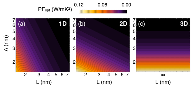
FIG. 2. (Color online) Optimum power factor PF_{\text{opt}} as a function of confinement length L and thermal de Broglie wavelength \Lambda plotted on a logarithmic scale for (a) 1D, (b) 2D, and (c) 3D systems.
