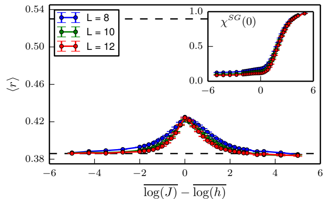
FIG. 1. Disorder averaged level statistics \langle r \rangle of H_F for the driven, disordered Ising model (4). \langle r \rangle approaches the Poisson limit of .386 with increasing L deep in the PM and SG phases, showing that these remain well localized. There is a peak in \langle r \rangle near the non-interacting critical point at \overline{\log \bar{J}} = \overline{\log \bar{h}} indicating partial delocalization, although the value still remains well below the COE value of .527. (inset): The SG diagnostic \chi^{SG} defined in (6) goes to 0 in the PM and approaches a non-zero value in the SG phase. All data is averaged over 2000 - 10^5 samples depending on L .
