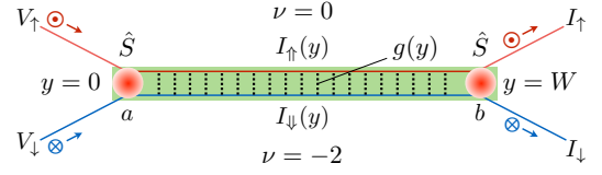
FIG. 3. (color online) The injection region. Charge currents entering vertices a and b redistribute according to scattering probability matrix \hat{S} . The inter-channel scattering inside the line junction is quantified by an effective conductance per unit length g(y) .
