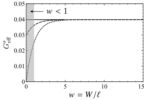
FIG. 4. Effective spin conductance G_{\text{eff}}^s \equiv I'_s/eV_- as a function of the aspect ratio w = W/\ell . The solid, dashed and dotted curves are, respectively, for full ( t = 0.5 ), partial ( t = 0.75 ) and no ( t = 1 ) inter-channel mixing at the vertices.
