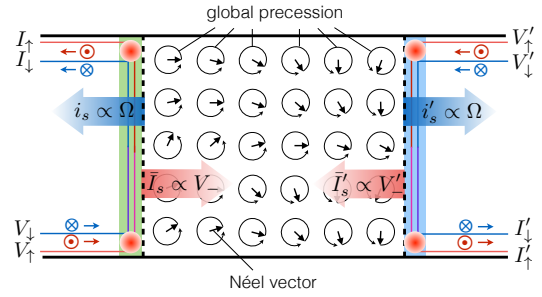
FIG. 2. (color online) A cartoon of the CAF in a dynamic superfluid state. The Néel vector rotates within the graphene plane about the z axis with a global precession frequency \Omega . The static contribution to spin current \bar{I}_s \propto V_- = V_\uparrow - V_\downarrow is injected into the CAF while the dynamic (spin-pumping) contribution i_s \propto \Omega pumps spin current back out into the edge. Two analogous contributions exist on the detection side.
