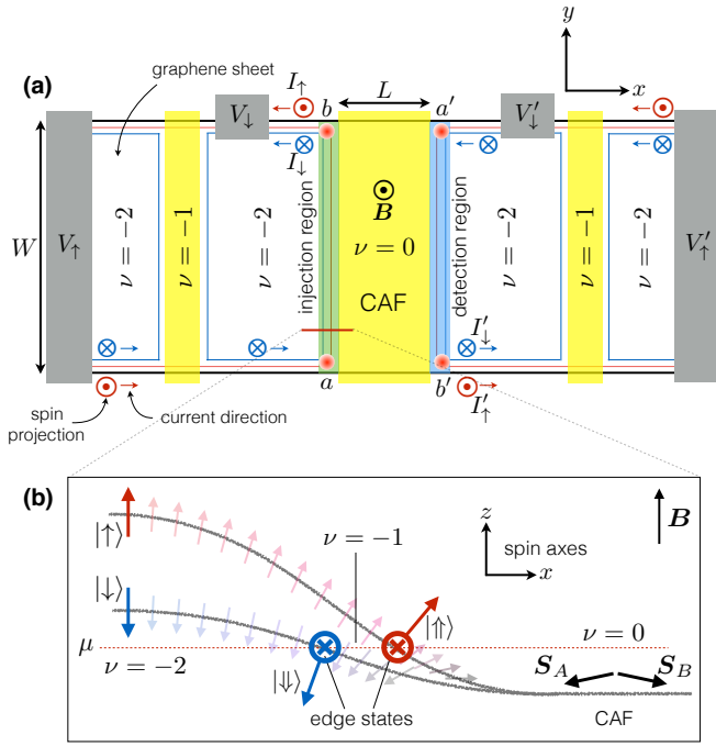
FIG. 1. (color online) Proposed setup for realizing and detecting superfluid spin transport through the \nu = 0 QH state of graphene. (a) Top view of the graphene Hall bar. Yellow regions are top gates and the grey regions denote ohmic contacts held at their respective voltages. Two independently biased spin-polarized edge channels on opposite sides of the \nu = 0 region are used to inject and detect spin current flowing through the CAF. The spin states of the \nu = -2 edge channels are polarized collinearly to the z axis outside of the injection and detection regions. (b) A cartoon energy diagram at a \nu = 0 to \nu = -2 transition region (across the bold red line). The spin axes are viewed from the side along the y direction. In the \nu = -2 region, energies of the two spin states, oppositely polarized along the z axis, are drawn; the Zeeman effect gives an energetic advantage to the spin-down state. In the \nu = 0 region, the two occupied branches of the CAF spectrum are shown. There, an external field in the positive z direction results in a ferromagnetic canting of spins in the negative z direction inside the antiferromagnet. Spin orientations of the chiral edge modes are intermediate between the up and down spin eigenstates within the \nu = -2 region (left side) and the canted spins within the CAF (right side). The black lines are merely a rough guide for the energies of the spin states in the transition region. The above illustration does not contain two other branches of the spectrum that are a part of the zLL but not essential for the edge physics in the transition region.
