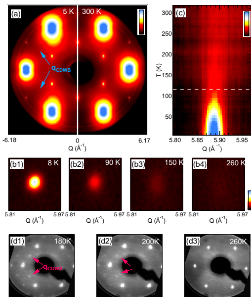
FIG. 2. Bulk and surface CDW transition. (a) High-energy x-ray diffraction patterns of the reciprocal lattice plane ( H K 0 ). The CDW superstructure peaks are marked by blue arrows (logarithmic color scale). (b) High-resolution diffraction patterns of the (\frac{9}{2} 0 0) CDW peak (linear color scale). (c) Plot of the temperature dependence of the CDW peak (linear color scale). The intensity is obtained by summing up the high-resolution diffraction patterns of the (\frac{9}{2} 0 0) peak along the transverse direction in (b), and is plotted along the longitudinal direction. (d) LEED images. Red arrows point to CDW superstructure peaks.
