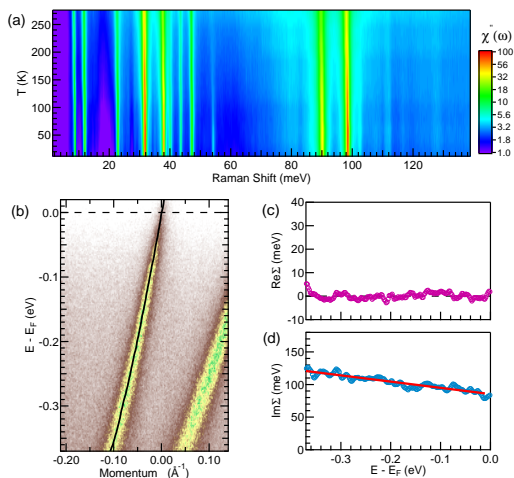
FIG. 3. (a) Temperature dependence of the Raman response in false color image (logarithmic scale) to emphasize a general trend of spectral weight suppression upon cooling due to gapping of the Fermi surface pockets. (b) Band crossing E_F at T = 260 K along same cut as in Fig. 1. The parabolic fit to the dispersion is plotted in black. (c) Real part of self-energy extracted from (b). (d) Imaginary part of self-energy extracted from (b). Red solid line is a linear fit.
