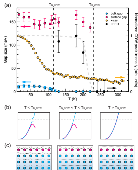
FIG. 4. Summary of the temperature-dependent CDW gap and band structure evolution. (a) Temperature dependence of surface (red solid circles) and bulk (blue solid circles) CDW gap. The surface gap is extracted from the back bending point of the surface band and the bulk gap is extracted from the leading edge shift of k_F EDCs (Fig. 1j). The gray solid line is a BCS-like temperature dependence with \Delta_0 = 12 meV. The integrated intensity of the CDW peak measured by x-ray diffraction (Fig. 2b) is shown with yellow solid circles. Black data points represent the intensity of CDW peaks measured by LEED. Dashed line is a guide to an eye. (b) Illustration of the surface (blue line) and bulk (red line) band dispersion. (c) Illustration of surface (red) and bulk (blue) CDW formation in real space. Dashed lines represent a density distribution of conducting electrons.
