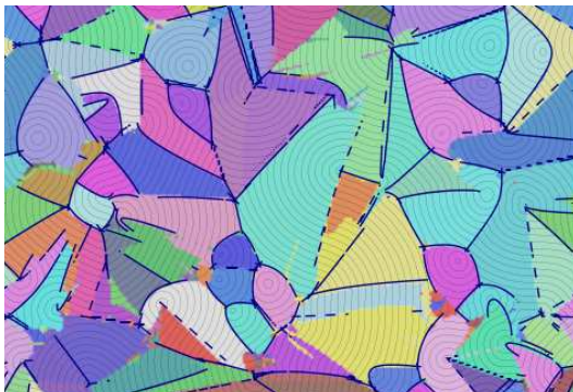
FIG. 4. Smectic microstructure of a two-dimensional planar boundary of a 3D simulation. The intersection of smectic layers and the section form sets of concentric circles, which are shown as thin black curves. The boundary between clusters (blue lines) are conics satisfying suitable compatibility conditions. Straight dashed lines separate domains whose ‘light cones’ are pointed in opposite directions and just miss tangency.
