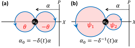
Figure 2. (color online) Sketch of the adiabatic paths of the components (a) |\!-\delta\alpha\rangle and (b) |\!-\delta^{-1}\alpha\rangle during the infinity gate.
