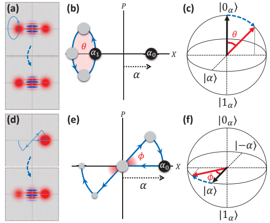
Figure 1. (color online) In the d = 2 cat-code, quantum information is encoded in the coherent states |\alpha_0(0)\rangle \equiv |\alpha\rangle and |\alpha_1(0)\rangle \equiv |-\alpha\rangle . (a) Wigner function sketch of the state before (top) and after (bottom) a loop gate acting on |-\alpha\rangle , depicting the path of |-\alpha\rangle during the gate (blue) and a shift in the fringes between |\pm\alpha\rangle . (b) Phase space diagram for the loop gate; X = \frac{1}{2}(\hat{a} + \hat{a}^\dagger) and P = -\frac{i}{2}(\hat{a} - \hat{a}^\dagger) . The parameter \alpha_1(t) is varied along a closed path (blue) of area A , after which the state |-\alpha\rangle gains a phase \theta = 2A relative to |\alpha\rangle . (c) Effective Bloch sphere of the |\pm\alpha\rangle qubit depicting the rotation caused by the d = 2 loop gate. Black arrow depicts initial state while red arrow is the state after application of the gate. The dotted blue arrow does not represent the path traveled since the states leave the logical space |\pm\alpha\rangle during the gate. (d-f) Analogous descriptions of the collision gate, which consists of reducing \alpha to 0, driving back to \alpha \exp(i\phi) , and rotating back to \alpha .
