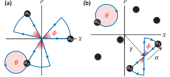
Figure 3. (color online) (a) Three-fold symmetric configuration of steady states |\alpha_\nu\rangle of Eq. (1) with d = 3 and depiction of a loop gate ( \theta ) acting on |\alpha_2\rangle and a collision gate ( \phi ) between all states. (b) Arbitrary configuration of steady states for d = 7 , depicting |\alpha_0\rangle undergoing a loop gate and |\alpha_1\rangle, |\alpha_2\rangle undergoing a displaced collision gate (see Supplementary Material).
