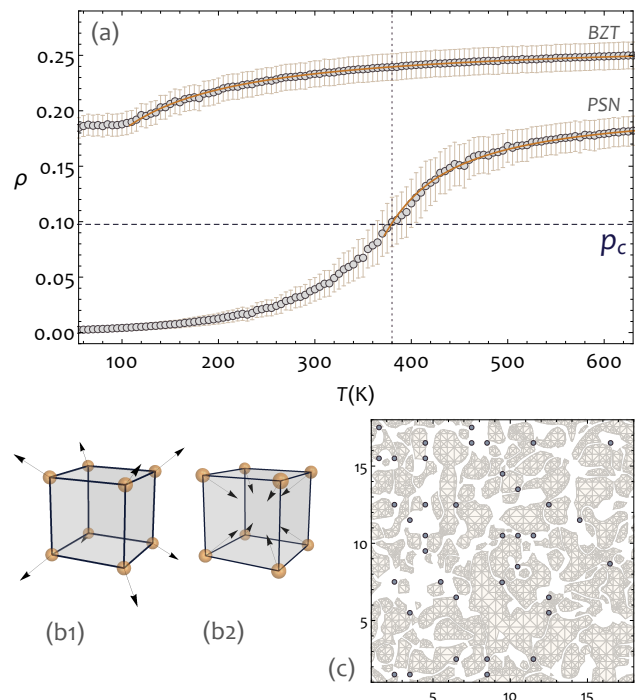
FIG. 1. (a) Temperature evolution of the density \rho of point topological defects (averaged over MC sweeps) for BZT and PSN. Solid lines correspond to exponential fits in the relaxor range. Horizontal dashed line indicates the site percolation threshold p_c . Vertical dashed line indicates the temperature at which the p_c line intersects the defects density of PSN ( \sim 380 K). (b) Schematic illustration of point topological defects at atomic scale. Yellow spheres correspond to B-sites to which local dipole moments (arrows) are allocated. The enclosed defect in the unit cell is (b1) a hedgehog corresponding to a source-like dipolar pattern or (b2) an antihedgehog corresponding to a sink-like dipolar pattern. (c) Transverse cross sectional view of PSN supercell for T=430 K showing the polar clusters (hatched regions) and the location of defects (circles) projected on the plane.
