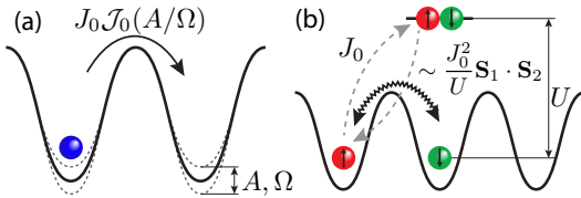
FIG. 1: Similarity between renormalisation of tunnelling, an interference effect induced virtually by an off-resonant drive (a), and Heisenberg interactions induced by virtual off-resonant interaction processes (b).
