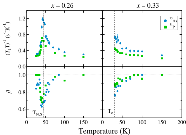
FIG. 1. (T_1T)^{-1} and \beta for ^{75}\text{As} ( \bullet ) and ^{31}\text{P} ( \square ) vs. temperature for x = 0.26 (underdoped) and x = 0.33 (optimal doping).
