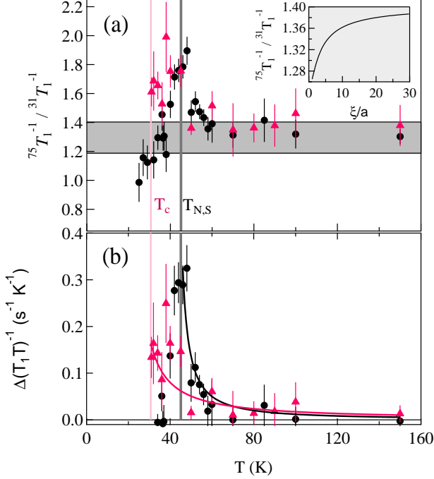
FIG. 2. (a) Ratio of the spin lattice relaxation rates of As to P ( {}^{75}T_1^{-1}/{}^{31}T_1^{-1} ) and (b) \Delta(T_1T)^{-1} vs. temperature for x = 0.26 ( \bullet ) and x = 0.33 ( \blacktriangle ). The gray horizontal region indicates the range of values for purely magnetic fluctuations. INSET: The theoretical ratio as a function of the antiferromagnetic correlation length, \xi . Solid lines in (b) are best fits as discussed in the text.
