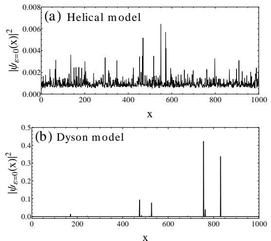
FIG. 2: Typical single-particle delocalized wave functions for the helical model [(a)] and the Dyson model [(b)] at energy \varepsilon = 0 (momentum space exact diagonalization [39]).
