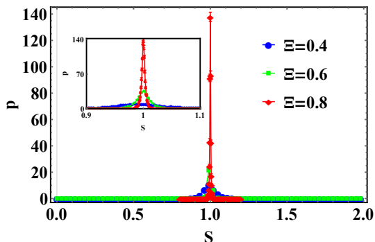
FIG. 1: \delta -type level spacing distribution p(s) for the noninteracting helical edge model, obtained by numerical diagonalization of the Hamiltonian Eq. (3b) in momentum space. We sample every other level to account for the Kramers degeneracy. Here s = |\varepsilon_n - \varepsilon_{n-2}|/\Delta is the normalized level spacing near energy \varepsilon_n , while \Delta is the average of |\varepsilon_n - \varepsilon_{n-2}| over the chosen set of levels. The parameter \Xi is the disorder correlation length in units of the inverse ultraviolet momentum cutoff [39, 49]. Inset: The broadening of the \delta -type distribution with different values of \Xi [39].
