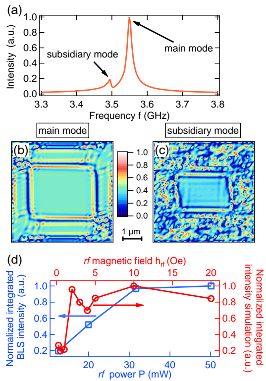
FIG. 5. Micromagnetic simulations: (a) The spectrum reveals two modes. Spatially-resolved magnetization distribution of the main mode, (b), and the less intense, subsidiary mode, (c). (d) The normalized integrated BLS intensity saturates at high excitation powers P , which is validated by micromagnetic simulations at large driving rf magnetic fields h_{rf} .
