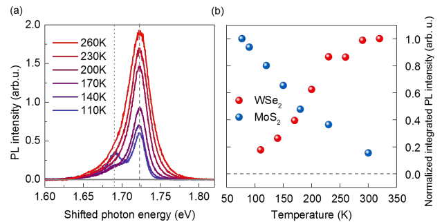
FIG. 1. (a) PL spectra of suspended monolayer WSe 2 at different temperatures, excited by pulsed 400 nm radiation. To facilitate comparison, the spectra at temperatures above 110 K have been shifted horizontally to align the A exciton emission feature (dashed line). The spectrum at 260 K has, for example, been blue shifted by 51 meV. (b) Comparison of temperature dependence of the time-integrated PL intensity of WSe 2 and MoS 2 . In both cases, the maximum intensity is normalized to unity. Excitation for the MoS 2 spectra was provided by a cw 532-nm laser.
