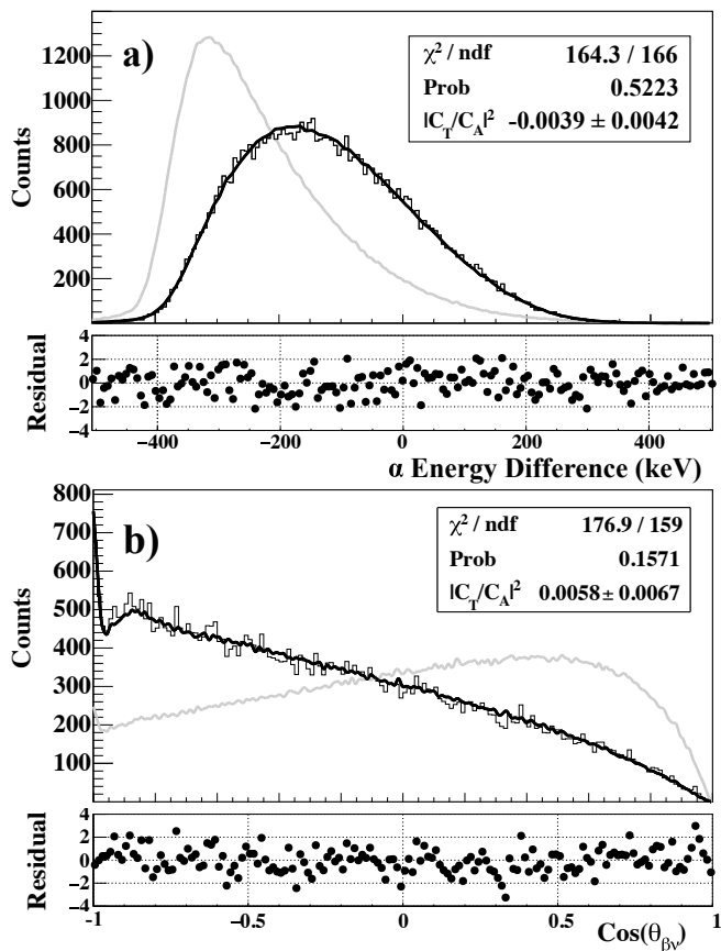
FIG. 2. Spectra from events with \beta and \alpha particles detected on the top and bottom detector. (a) Energy difference along with the fit to the simulated spectrum and the normalized residual. (b) The reconstructed \cos(\theta_{\beta\nu}) spectrum for the same events with a fit to the simulated spectrum and the normalized residual. The gray curves show the expected spectra for a pure T interaction.
