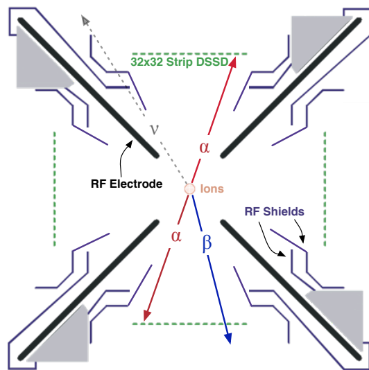
FIG. 1. Cross-sectional view of the BPT and detector system in the RF plane. The direction of the emitted \alpha s and \beta s is determined by the vector between the trap center and detector pixels.
