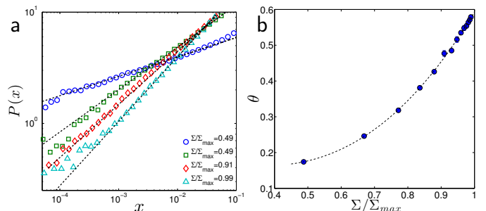
FIG. 2. (a) Distribution of local stability P(x) for \Sigma/\Sigma_{max} = 0.49 to 0.99 in the stress-control protocol for N = 1024^2 in the case \Sigma_{max} = \Sigma_c . The dashed lines are direct fits of the form P(x) \sim x^\theta , from which we extract \theta . This quantity is shown in (b). The dashed line is the interpolation using a third order polynomial fit.
